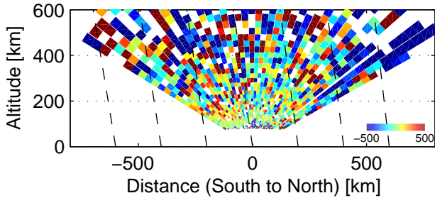
Vi, 74546–74754 UT, 12/3, 2005
