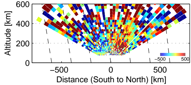
Vi, 85610–85818 UT, 12/3, 2005
