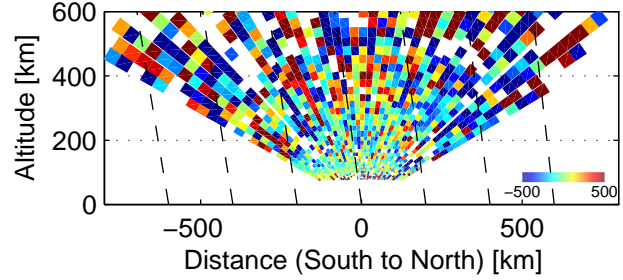
Vi, 82202–82410 UT, 12/3, 2005
