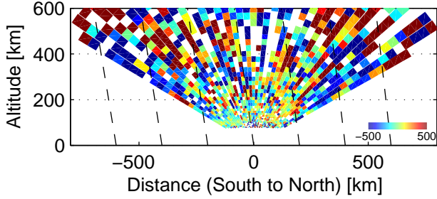
Vi, 84114–84322 UT, 12/3, 2005
