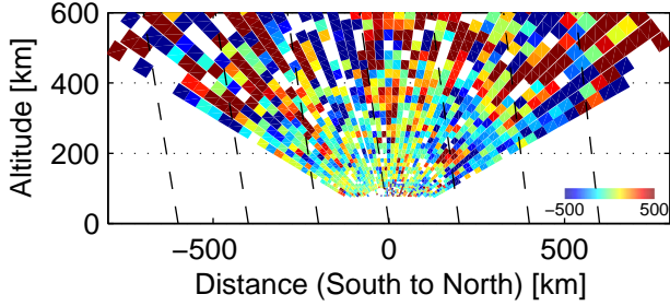
Vi, 81954–82202 UT, 12/3, 2005
