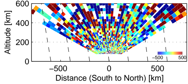
Vi, 84322–84530 UT, 12/3, 2005
