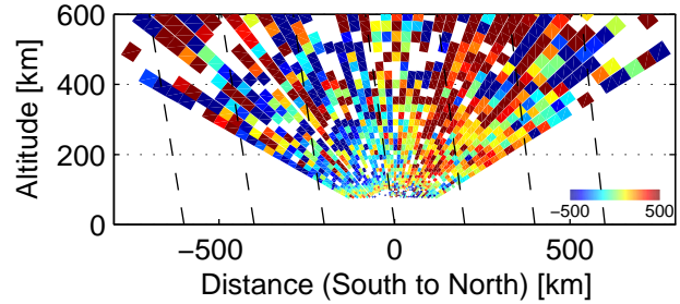
Vi, 83450–83658 UT, 12/3, 2005
