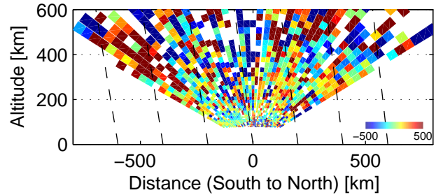
Vi, 85154–85402 UT, 12/3, 2005
