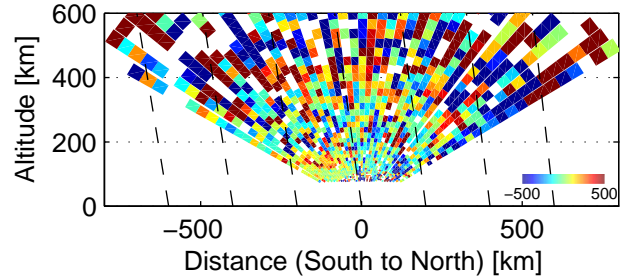
Vi, 74338–74546 UT, 12/3, 2005
