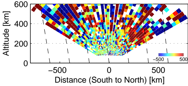
Vi, 81538–81746 UT, 12/3, 2005
