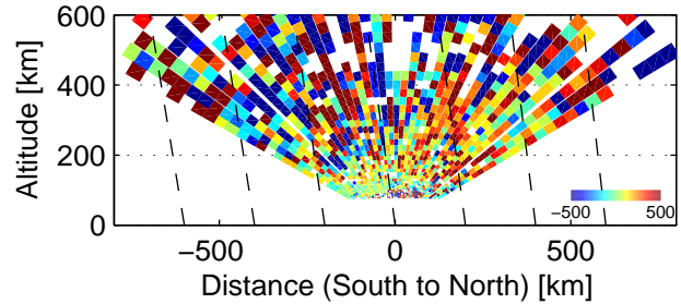
Vi, 83034–83242 UT, 12/3, 2005
