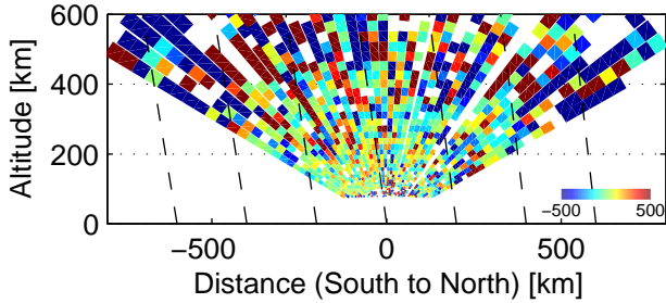
Vi, 75002–75210 UT, 12/3, 2005
