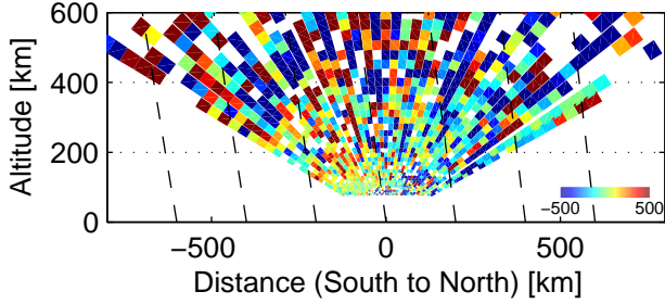
Vi, 73714–73922 UT, 12/3, 2005
