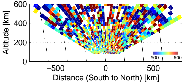
Vi, 85402–85610 UT, 12/3, 2005
