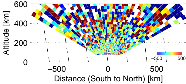
Vi, 74130–74338 UT, 12/3, 2005
