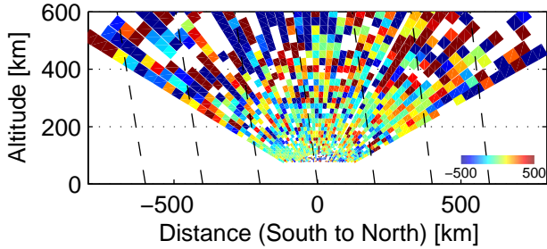
Vi, 82410–82618 UT, 12/3, 2005
