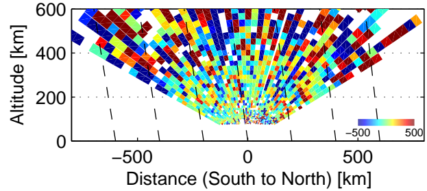
Vi, 75210–75418 UT, 12/3, 2005
