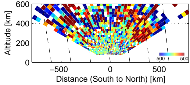
Vi, 81746–81954 UT, 12/3, 2005
