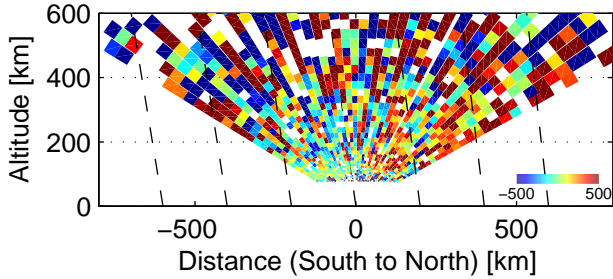
Vi, 84530–84738 UT, 12/3, 2005
