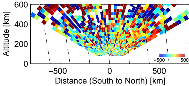
Vi, 82826–83034 UT, 12/3, 2005
