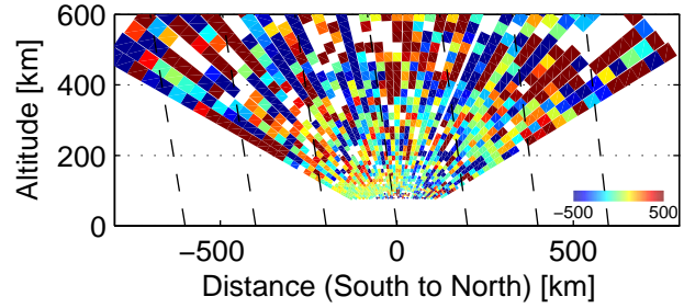
Vi, 73506–73714 UT, 12/3, 2005
