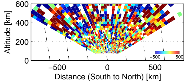
Vi, 84738–84946 UT, 12/3, 2005
