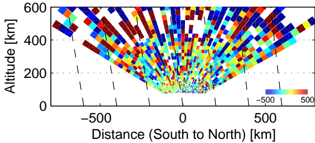
Vi, 84946–85154 UT, 12/3, 2005
