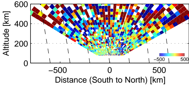
Vi, 73258–73506 UT, 12/3, 2005
