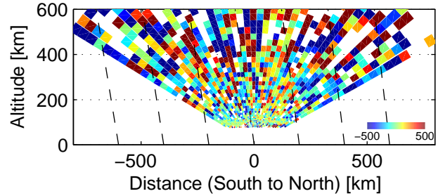
Vi, 94133–94341 UT, 12/4, 2005
