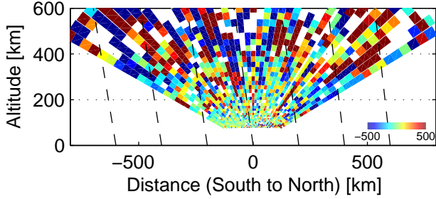
Vi, 93509–93717 UT, 12/4, 2005
