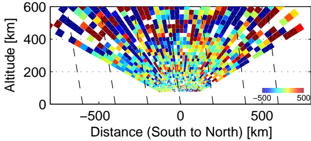
Vi, 93925–94133 UT, 12/4, 2005
