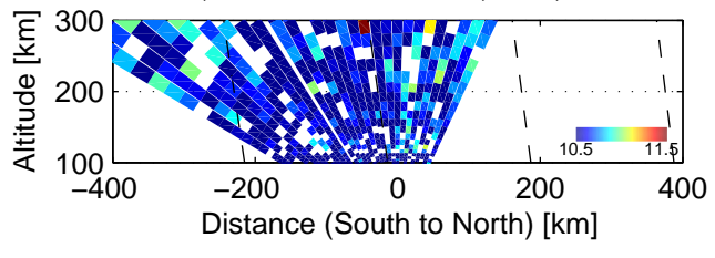
Ne, 125830–130000 UT, 12/5, 2005
