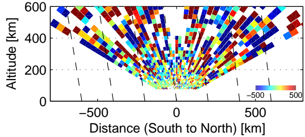
Vi, 73830–74038 UT, 12/5, 2005
