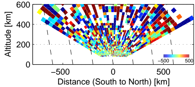
Vi, 85518–85726 UT, 12/5, 2005
