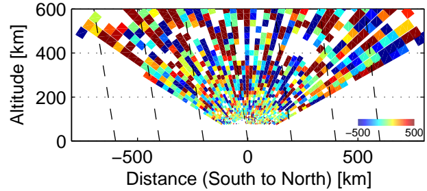
Vi, 85934–90142 UT, 12/5, 2005
