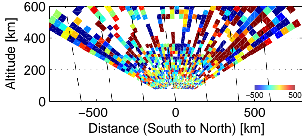
Vi, 84854–85102 UT, 12/5, 2005
