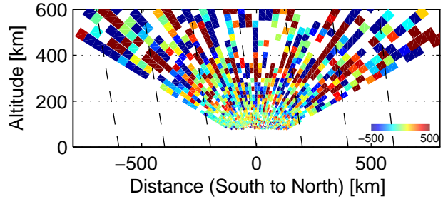
Vi, 74702–74910 UT, 12/5, 2005
