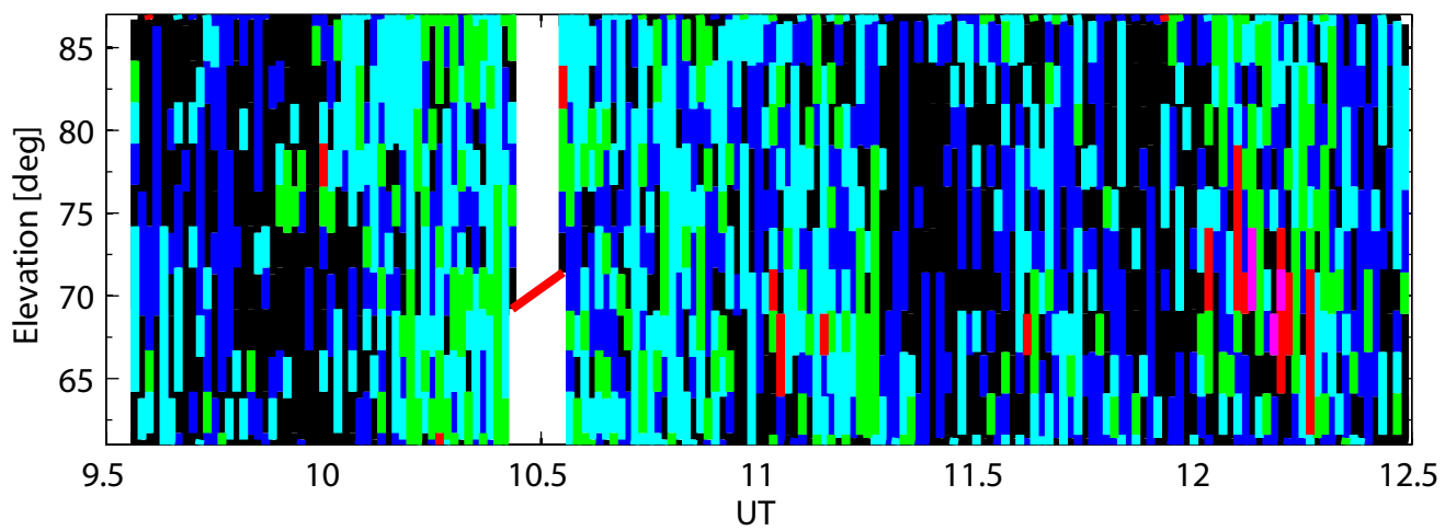
2007-02-26, 200 km altitude
