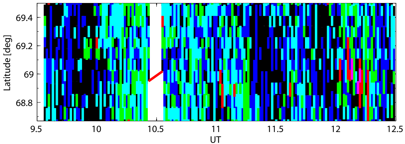
2007-02-26, 200 km altitude
