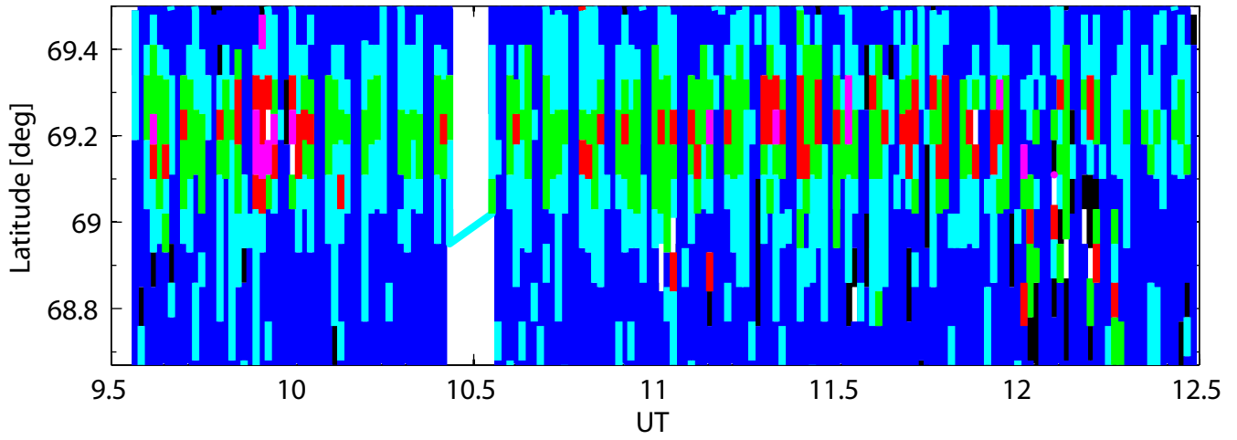
2007-02-26, 200 km altitude
