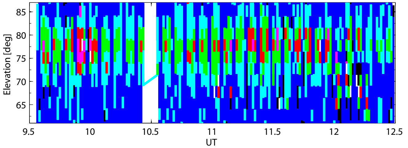
2007-02-26, 200 km altitude
