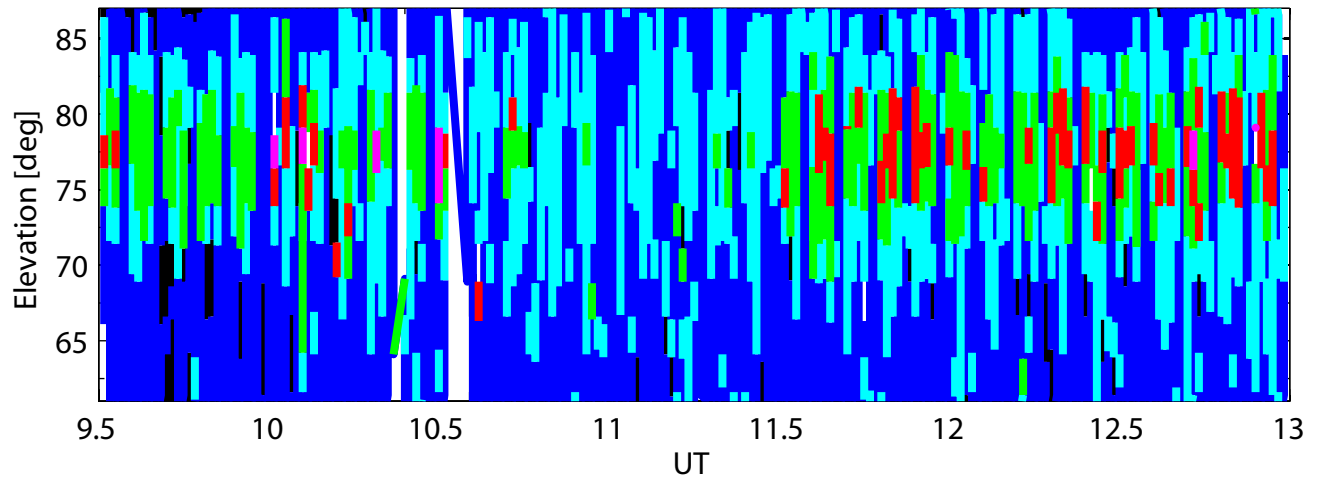
2007-02-27, 200 km altitude
