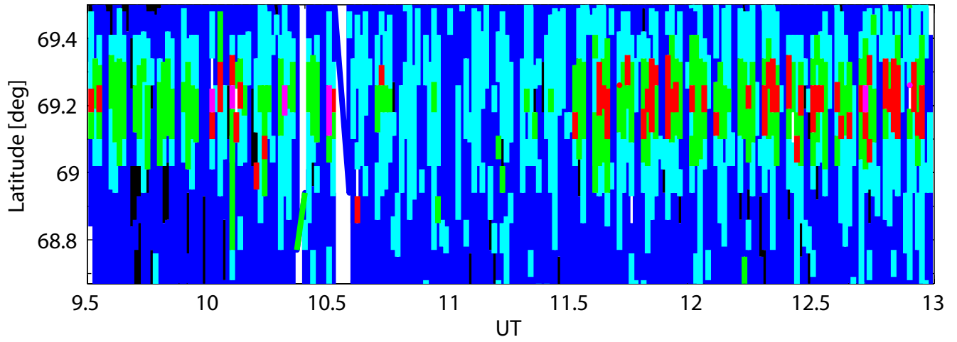
2007-02-27, 200 km altitude
