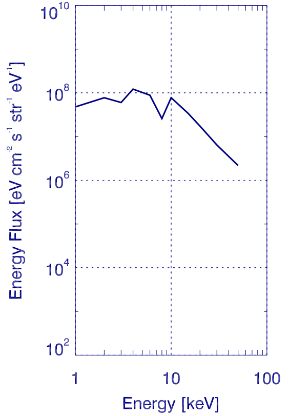
EISCAT 000600
