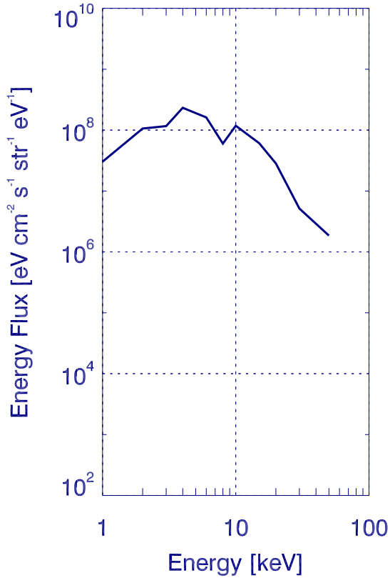
EISCAT 001900
