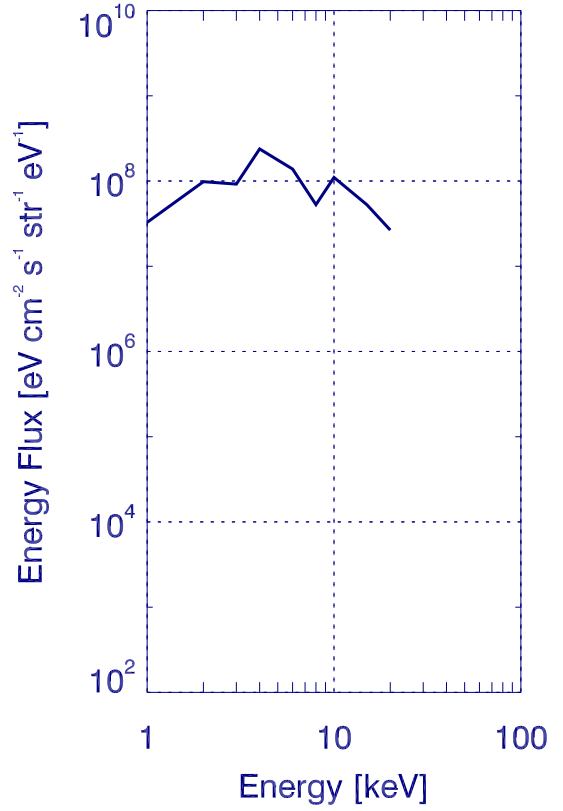
EISCAT 002200
