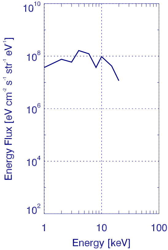
EISCAT 003100
