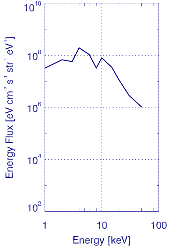
EISCAT 004600
