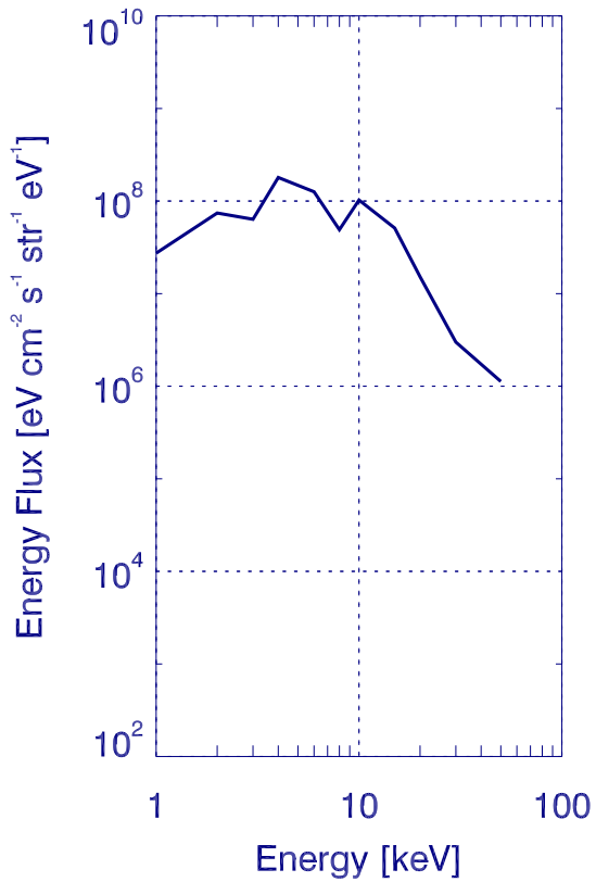
EISCAT 002700
