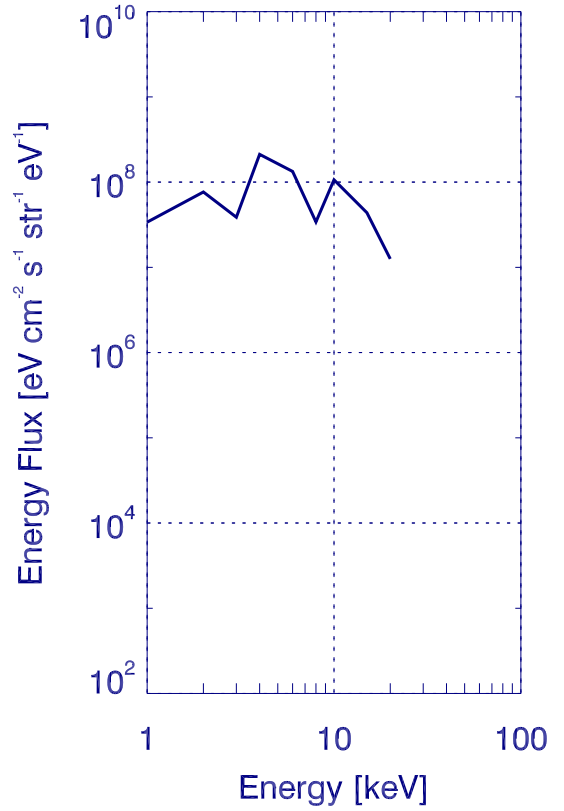
EISCAT 003200
