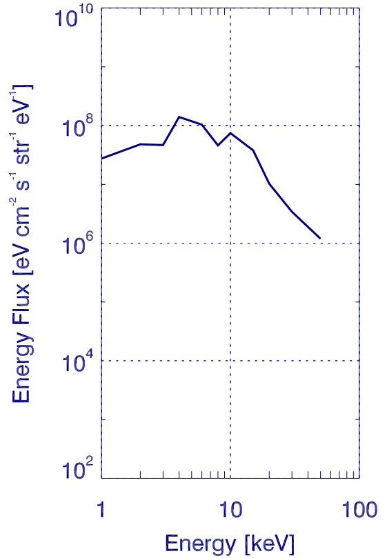
EISCAT 004800
