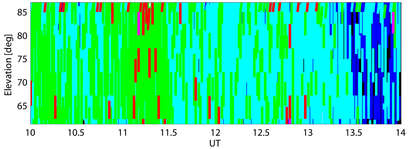
2008-03-06, 200 km altitude, Ne
