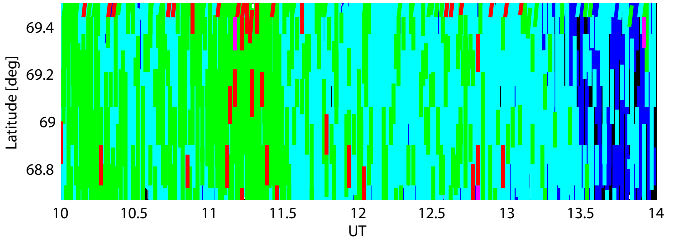
2008-03-06, 200 km altitude, Ne
