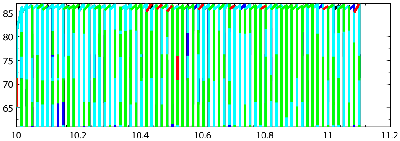
2008-03-07, 200 km altitude, Ne
