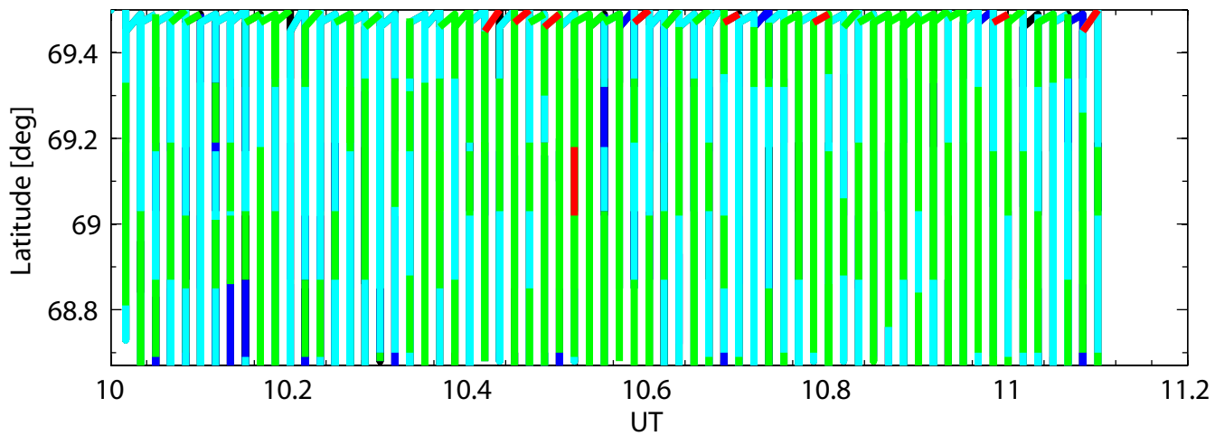
2008-03-07, 200 km altitude, Ne
