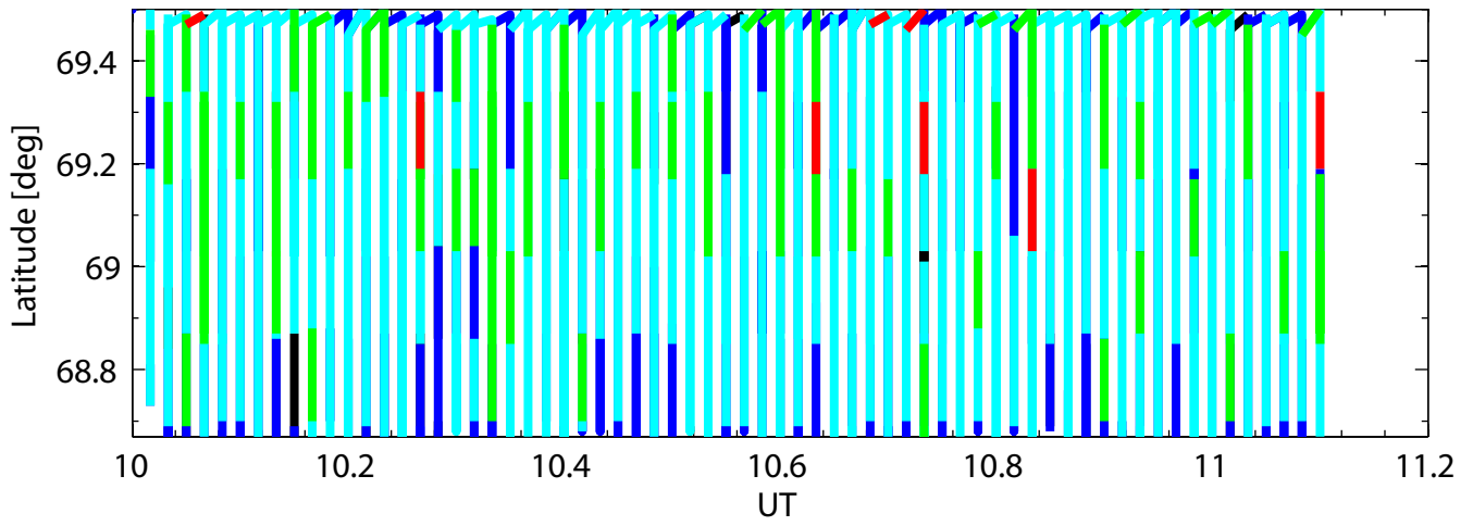
2008-03-07, 200 km altitude, Te
