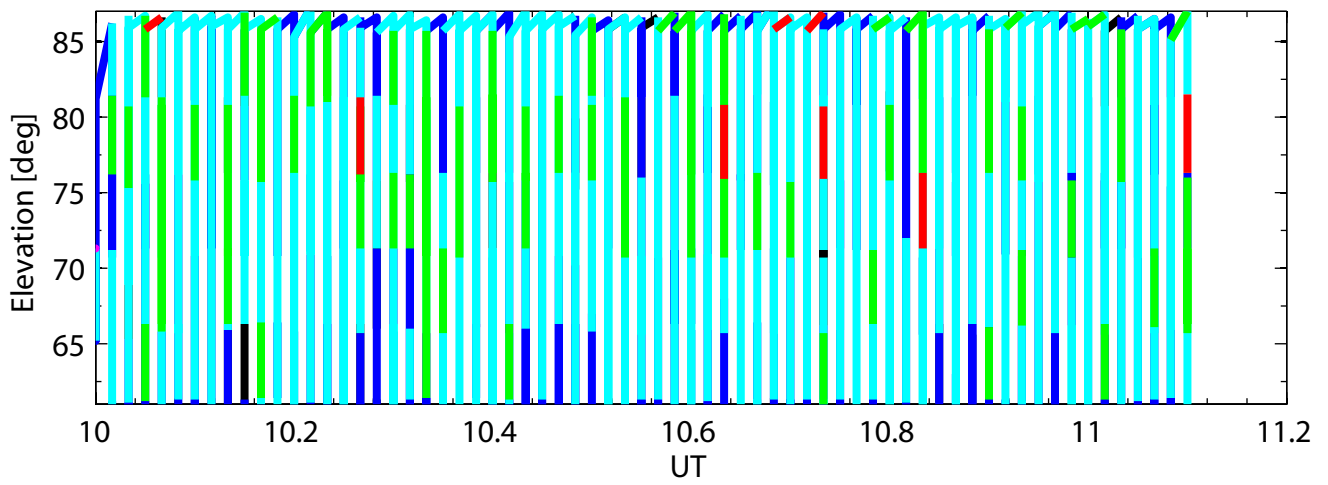
2008-03-07, 200 km altitude, Te
