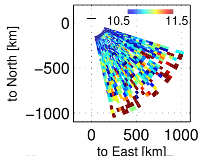
Ne, 102000 – 102403 UT, 20171201
