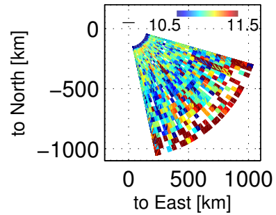
Ne, 71600 – 72003 UT, 20171201
