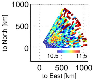
Ne, 105603 – 105954 UT, 20171221
