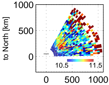
Ne, 103203 – 103600 UT, 20171221
