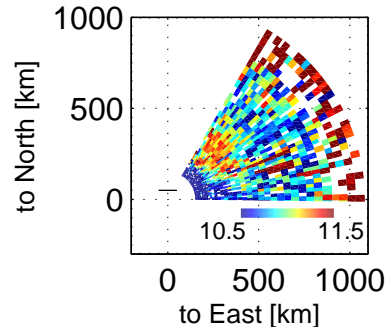
Ne, 102000 – 102403 UT, 20171221
