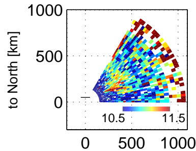
Ne, 105200 – 105603 UT, 20171221
