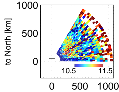
Ne, 103600 – 104003 UT, 20171221
