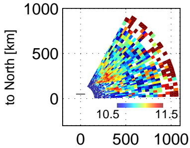
Ne, 104003 – 104400 UT, 20171221
