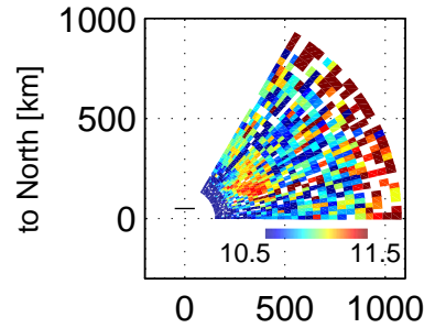
Ne, 104400 – 104803 UT, 20171221
