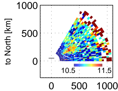
Ne, 102000 – 102403 UT, 20171221
