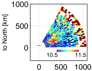
Ne, 105603 – 105954 UT, 20171221
