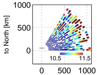
Ne, 101603 – 101758 UT, 20171222
