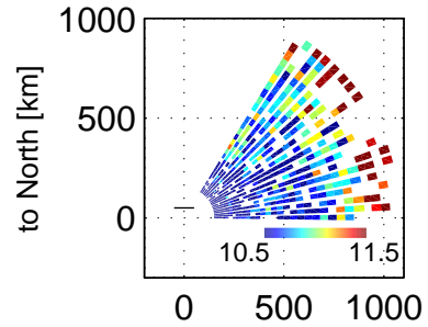
Ne, 103203 – 103358 UT, 20171222
