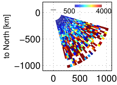
Te, 91203 – 91600 UT, 20171201
