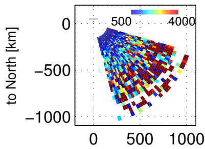
Te, 93200 – 93603 UT, 20171201
