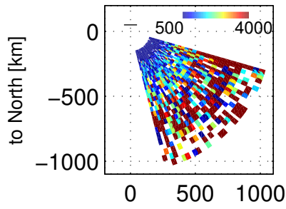
Te, 92003 – 92400 UT, 20171201
