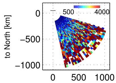
Te, 93603 – 94000 UT, 20171201
