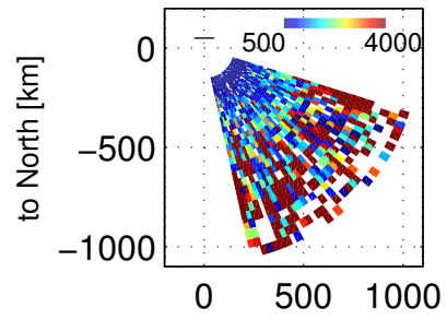
Te, 92400 – 93200 UT, 20171201
