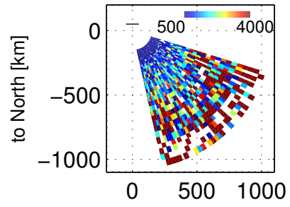
Te, 91600 – 92003 UT, 20171201
