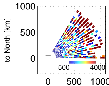
Te, 101603 – 101758 UT, 20171222
