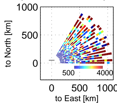
Te, 102000 – 102202 UT, 20171222
