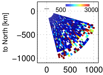
Ti, 104003 – 104400 UT, 20171201
