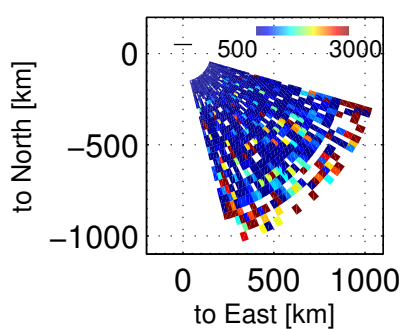
Ti, 85603 – 90000 UT, 20171201
