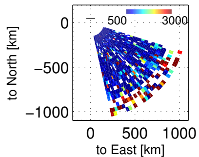
Ti, 74000 – 74403 UT, 20171201
