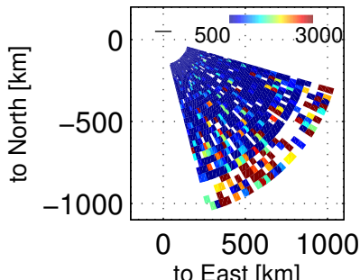
Ti, 72003 – 72400 UT, 20171201
