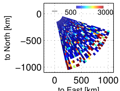
Ti, 74000 – 74403 UT, 20171201
