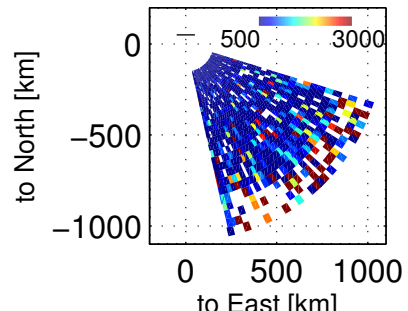
Ti, 72400 – 72803 UT, 20171201
