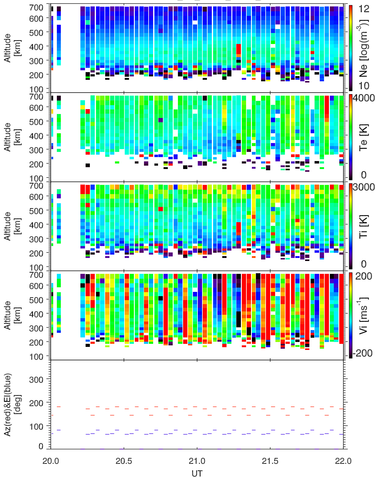
EISCAT 1998-03-27_20_22UT_gup0_ant@32m.
