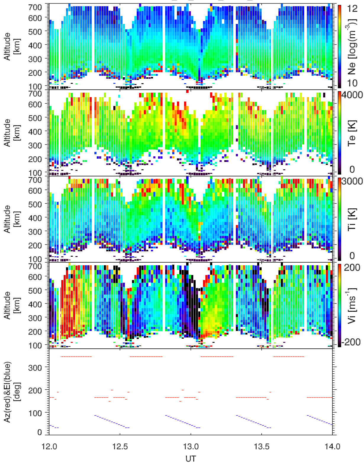
EISCAT 1998-04-27_12_14UT_gup0_ant@32m.
