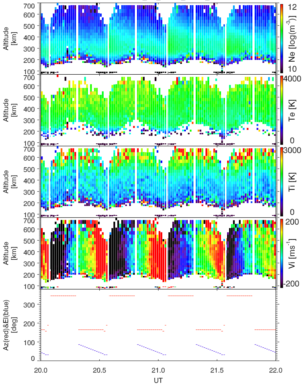
EISCAT 1998-04-27_20_22UT_gup0_ant@32m.
