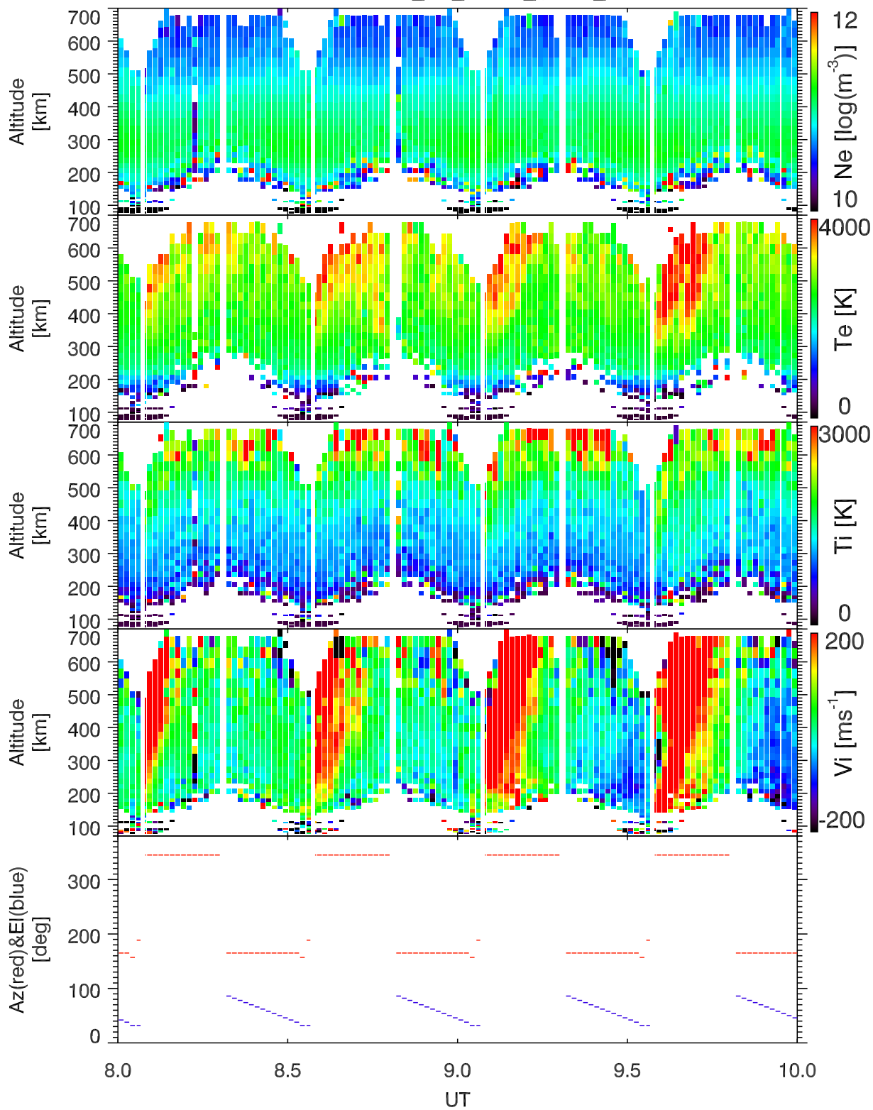
EISCAT 1998-04-29_08_10UT_gup0_ant@32m.
