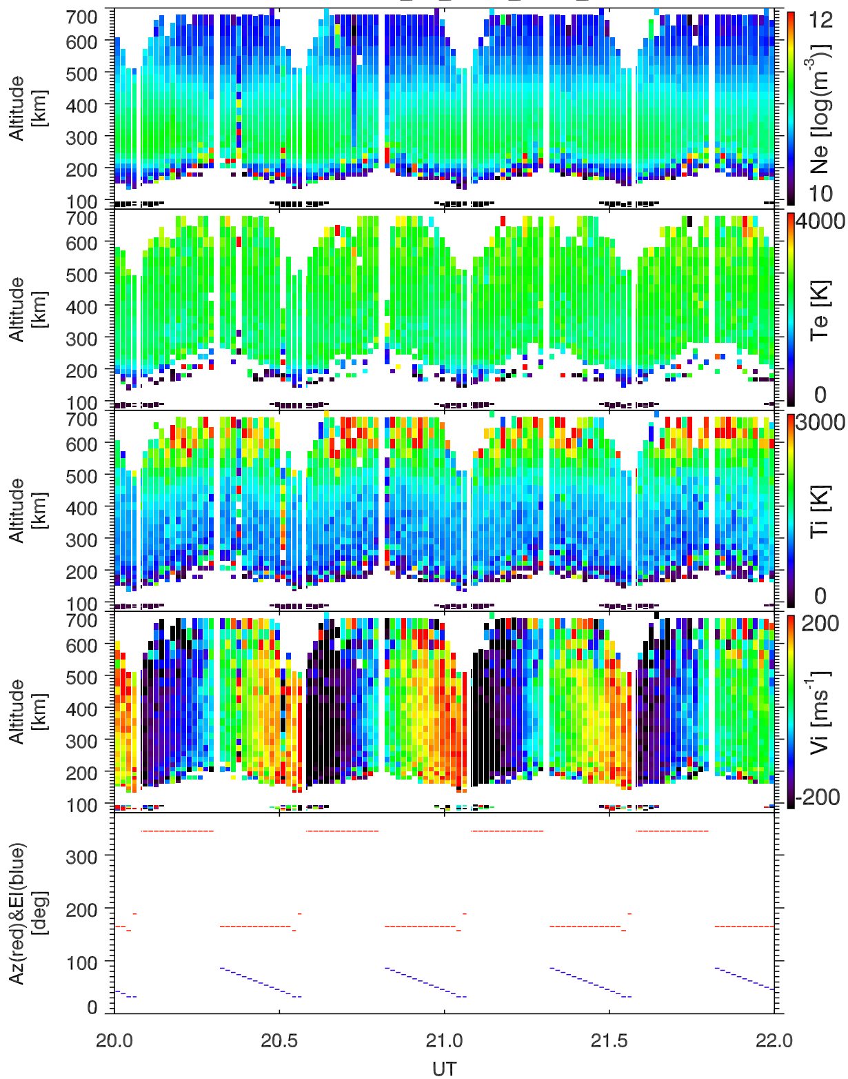
EISCAT 1998-04-29_20_22UT_gup0_ant@32m.
