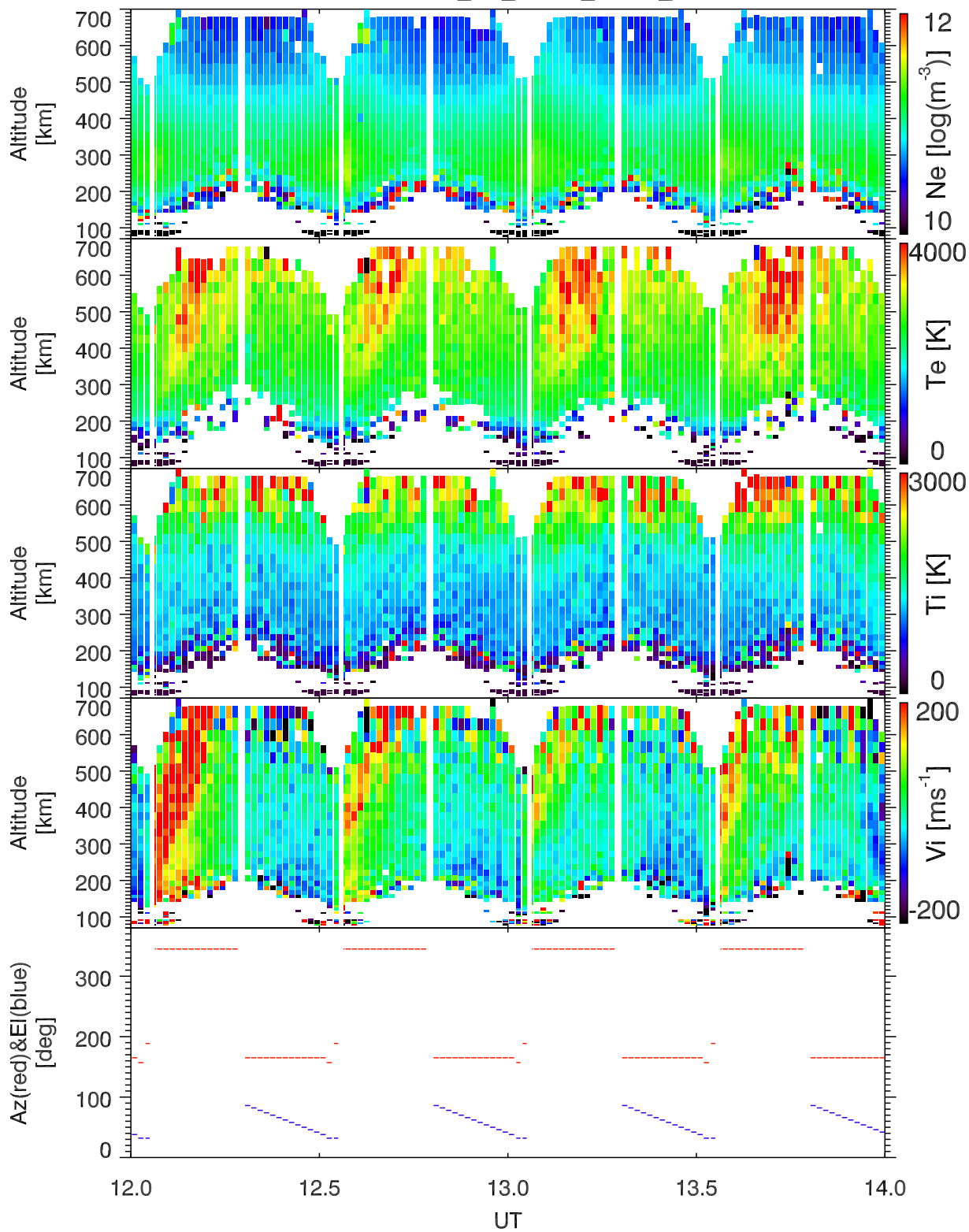
EISCAT 1998-04-30_12_14UT_gup0_ant@32m.
