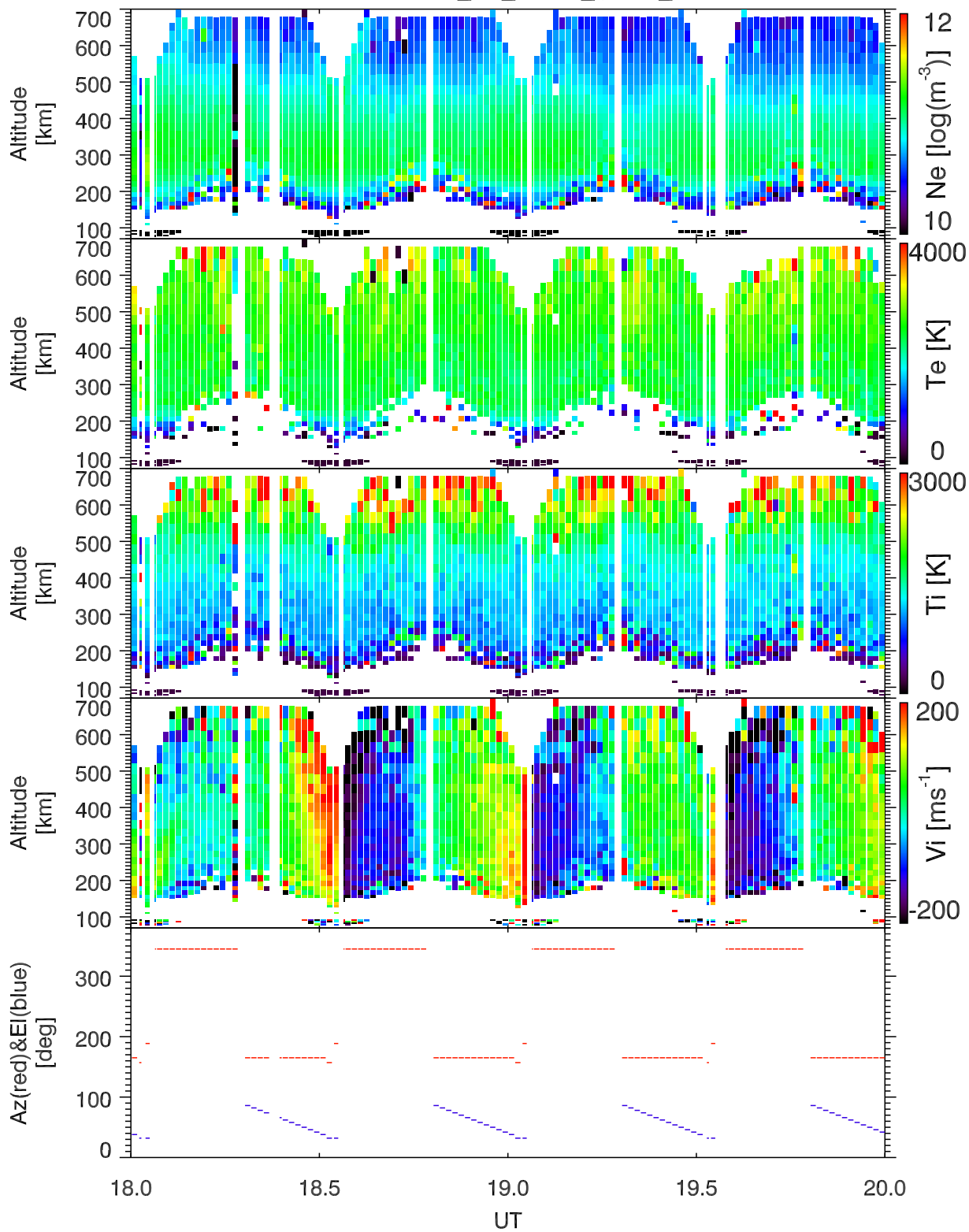
EISCAT 1998-04-30_18_20UT_gup0_ant@32m.
