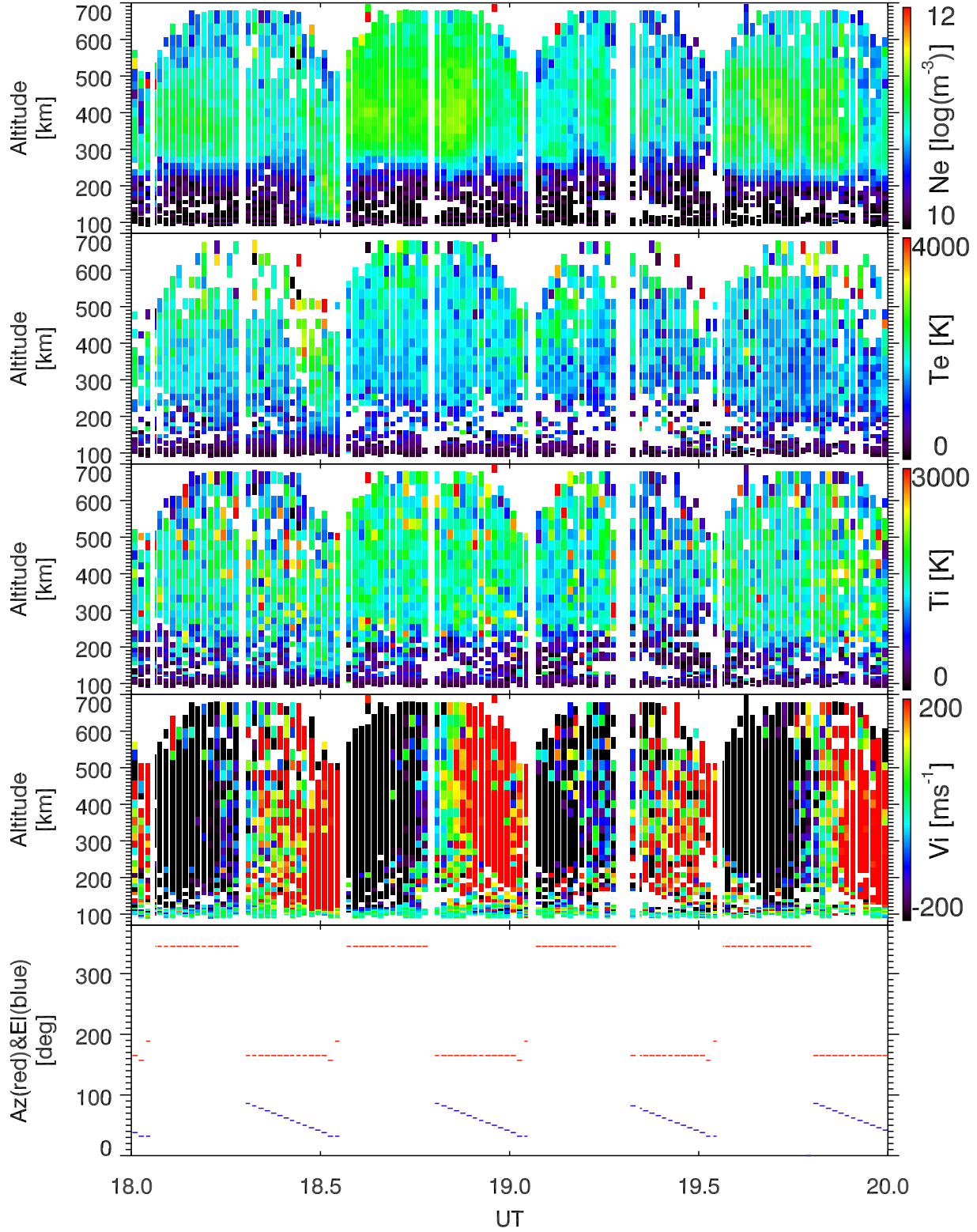
EISCAT 1998-10-19_18_20UT_gup3c_ant@32m.
