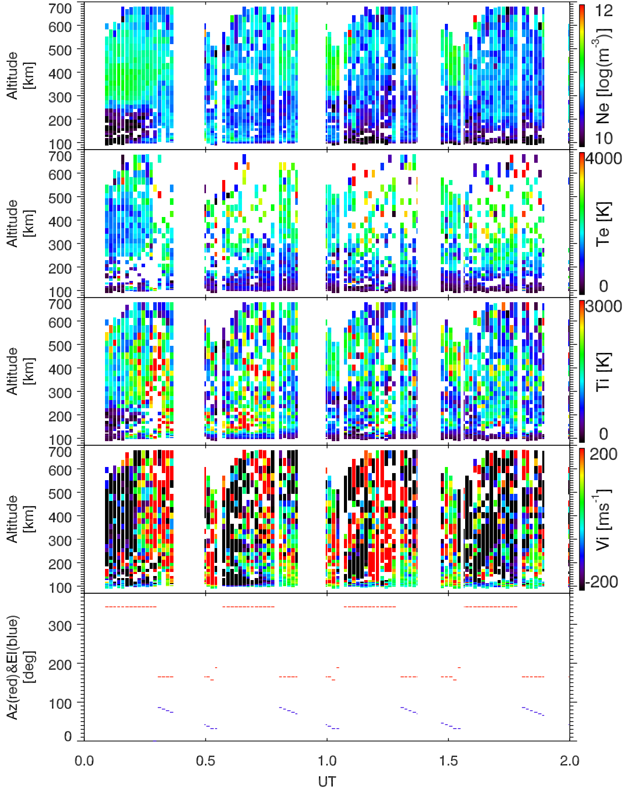
EISCAT 1998-10-21_00_02UT_gup3c_ant@32m.
