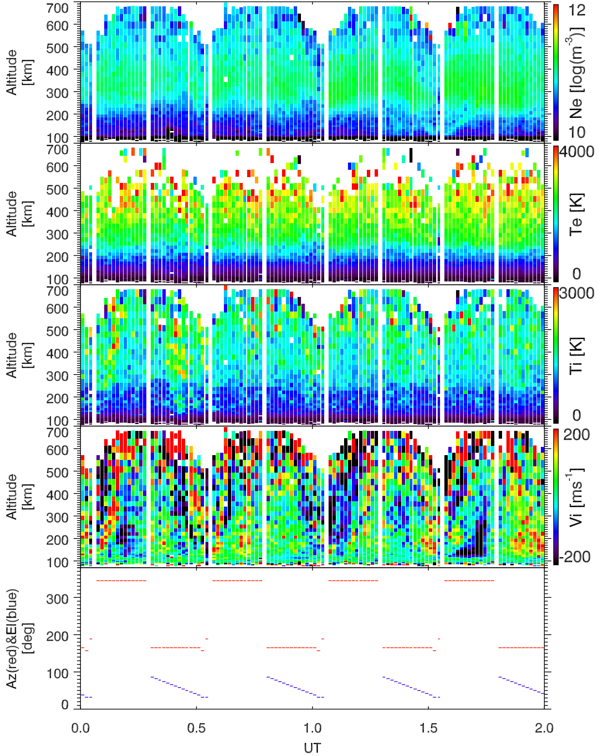
EISCAT 1999-04-21_00_02UT_gup3c_ant@32m.
