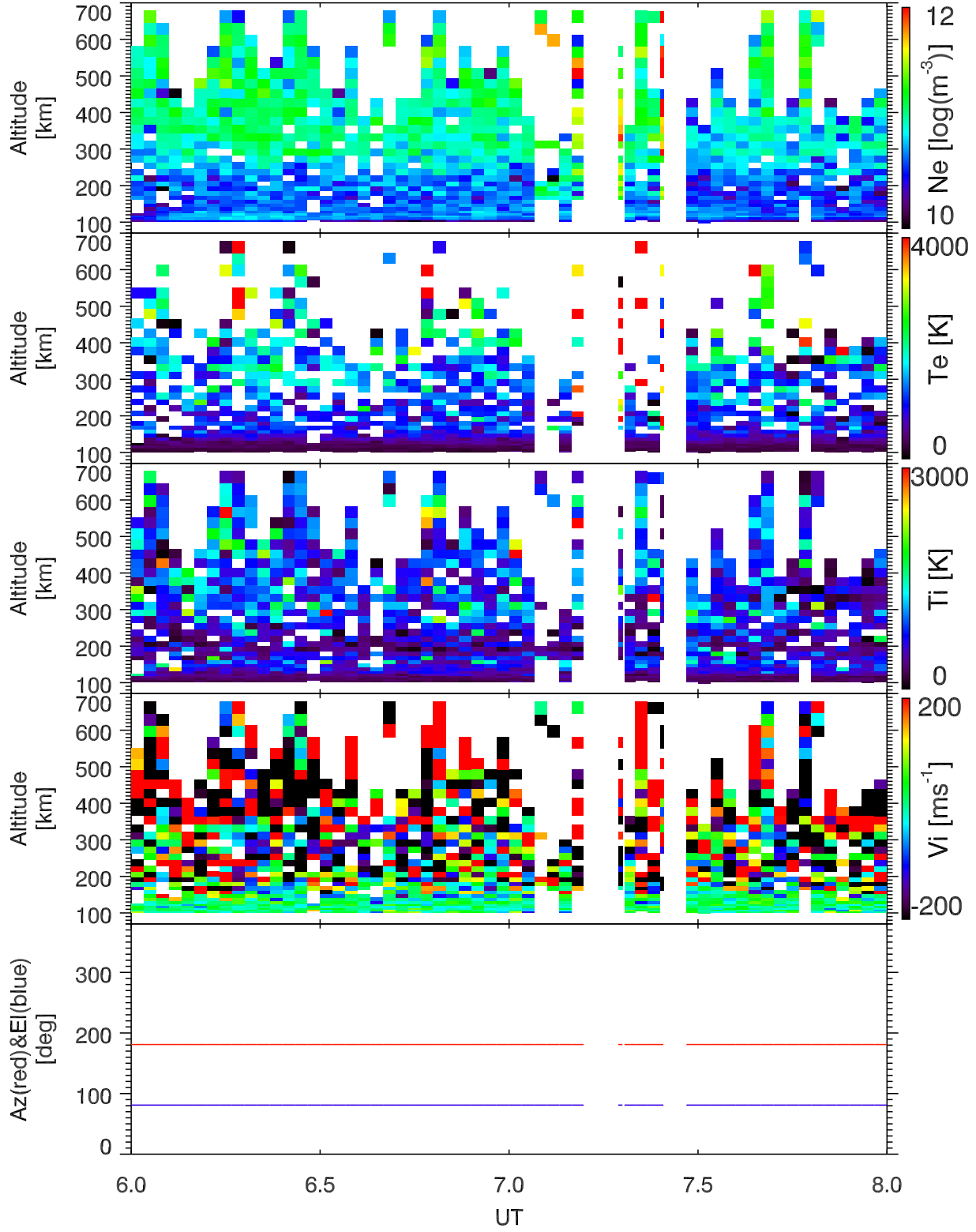
EISCAT 2000-01-07_06_08UT_gup3c_120@42m.
