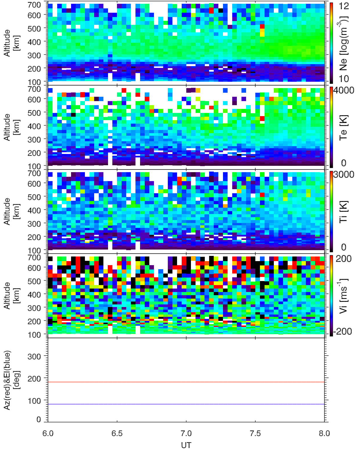
EISCAT 2000-02-08_06_08UT_gup3c_120@42m.
