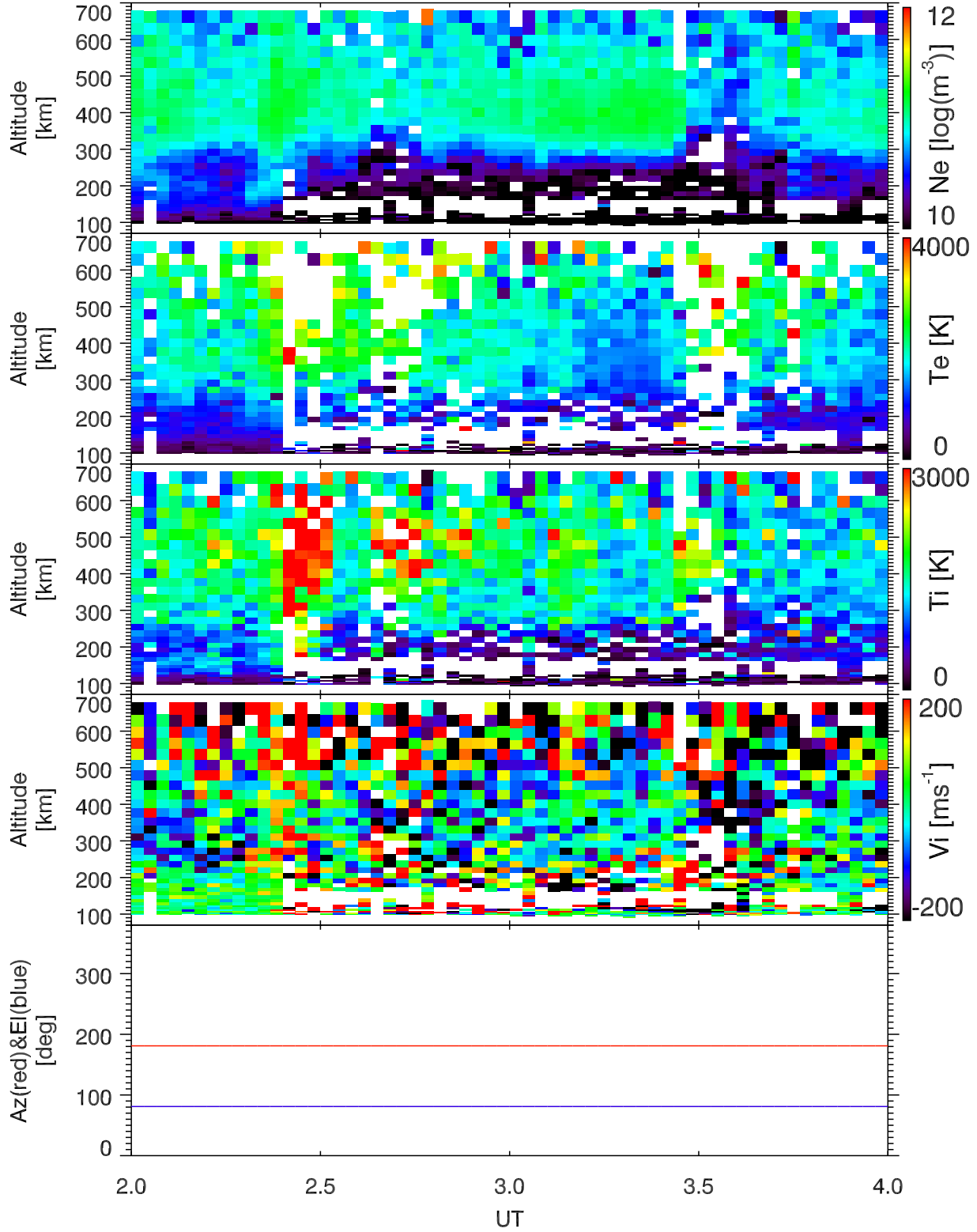
EISCAT 2000-02-10_02_04UT_gup3c_120@42m.
