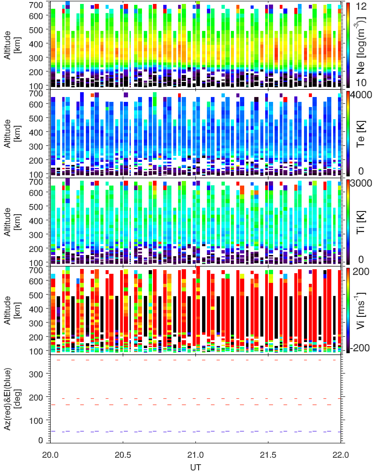
EISCAT 2000-03-14_20_22UT_gup3c_ant@32m.
