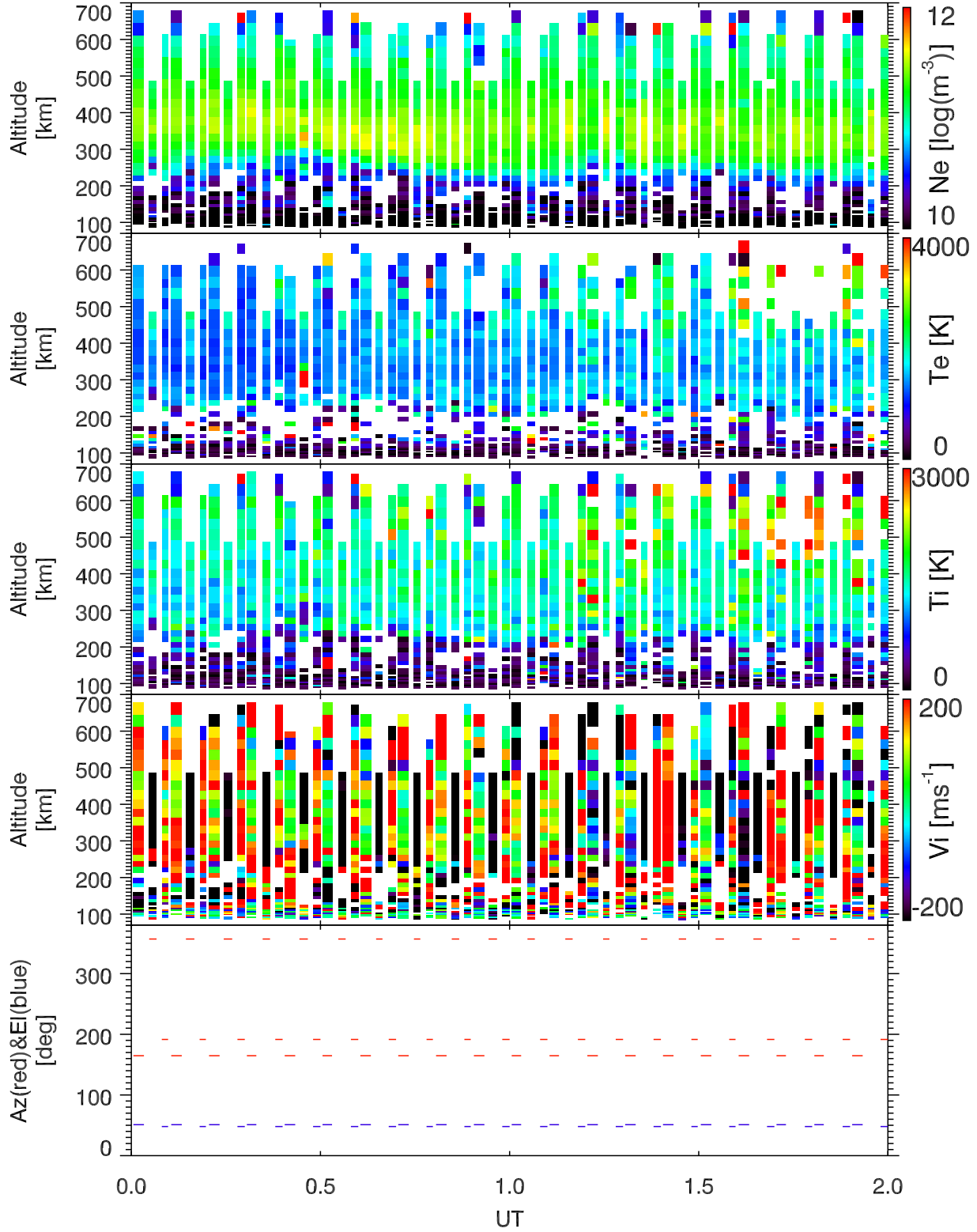
EISCAT 2000-03-15_00_02UT_gup3c_ant@32m.
