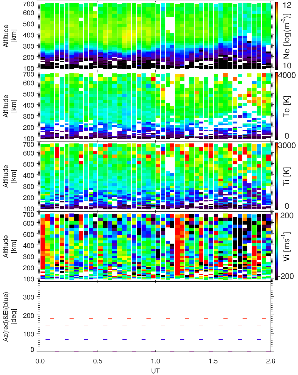
EISCAT 2000-03-19_00_02UT_gup3c_ant@32m.
