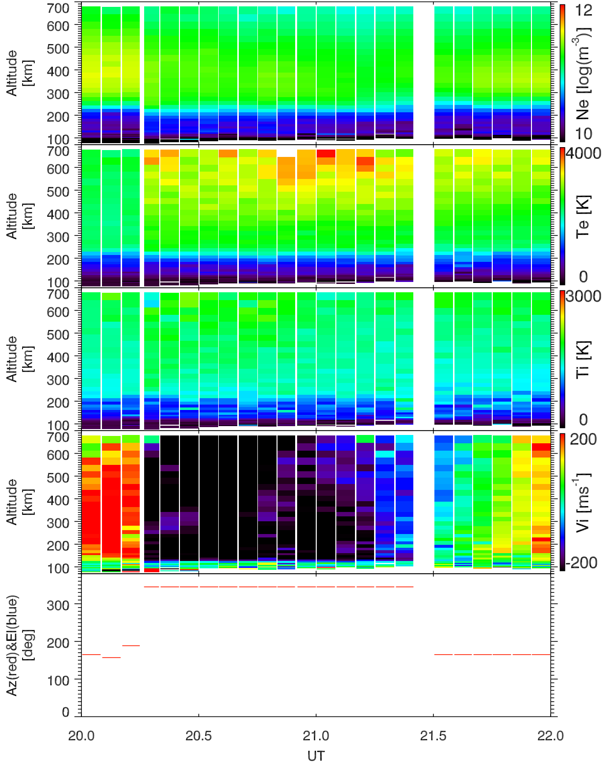
EISCAT 2000-04-11_20_22UT_tau0_ant@32m.
