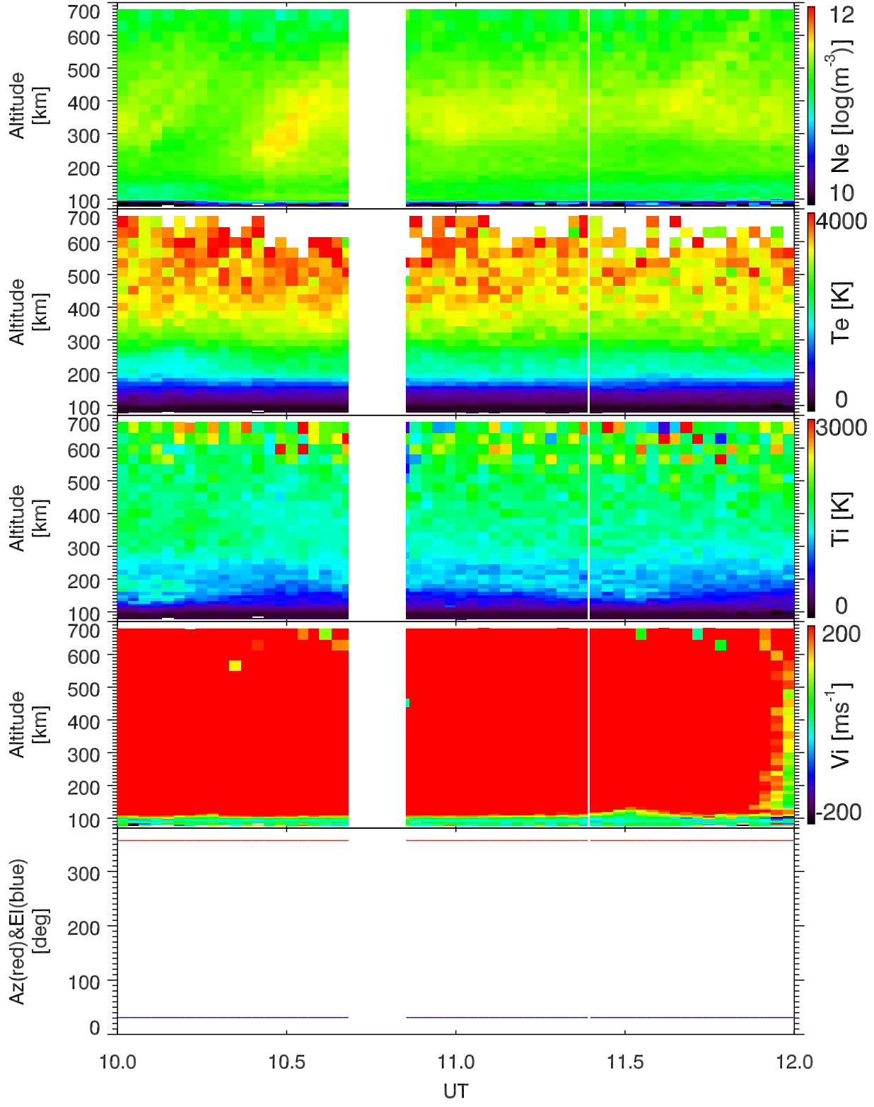
EISCAT 2000-07-14_10_12UT_tau0_120@32m.
