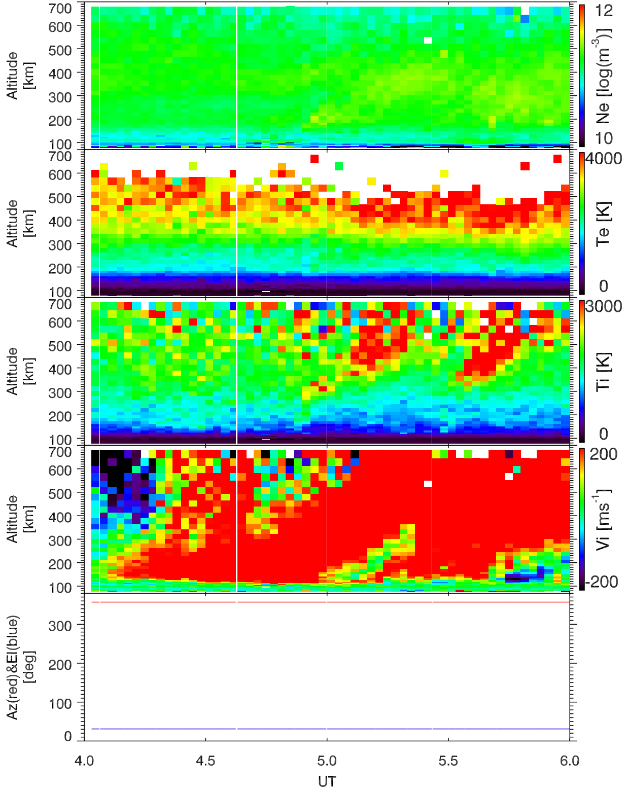
EISCAT 2000-07-15_04_06UT_tau0_120@32m.
