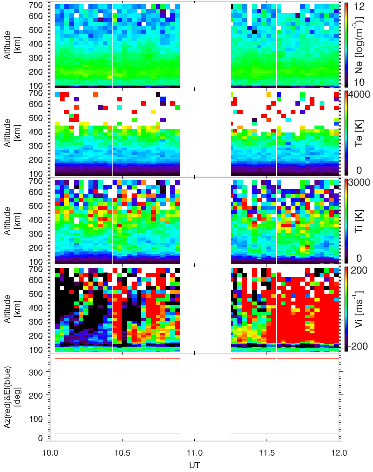
EISCAT 2000-07-16_10_12UT_tau0_120@32m.
