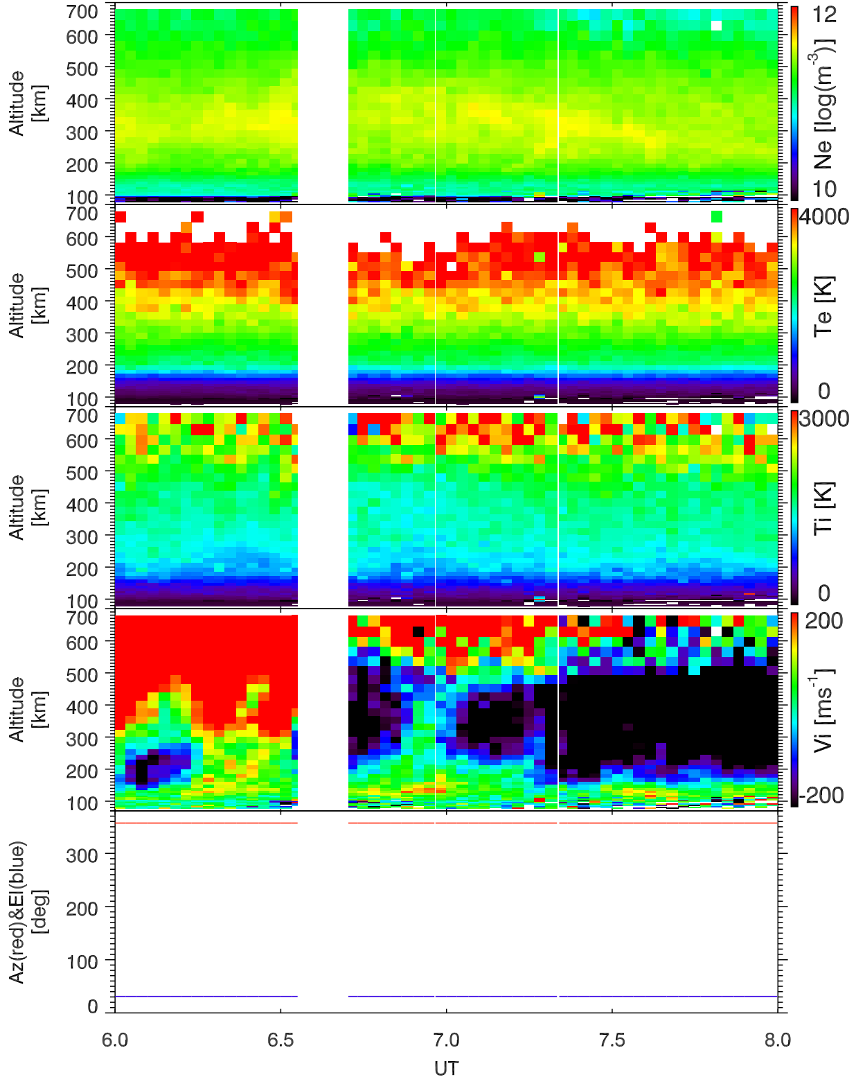
EISCAT 2000-07-17_06_08UT_tau0_120@32m.
