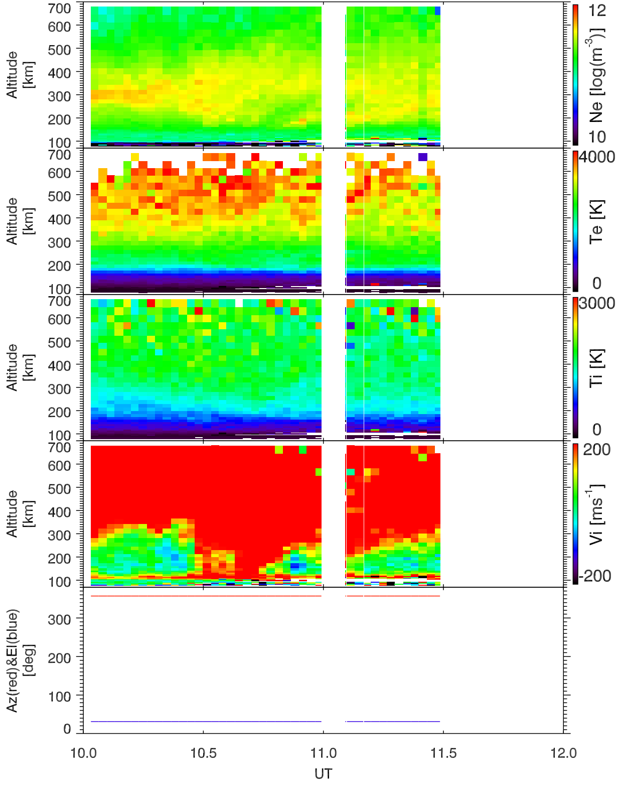
EISCAT 2000-07-18_10_12UT_tau0_120@32m.
