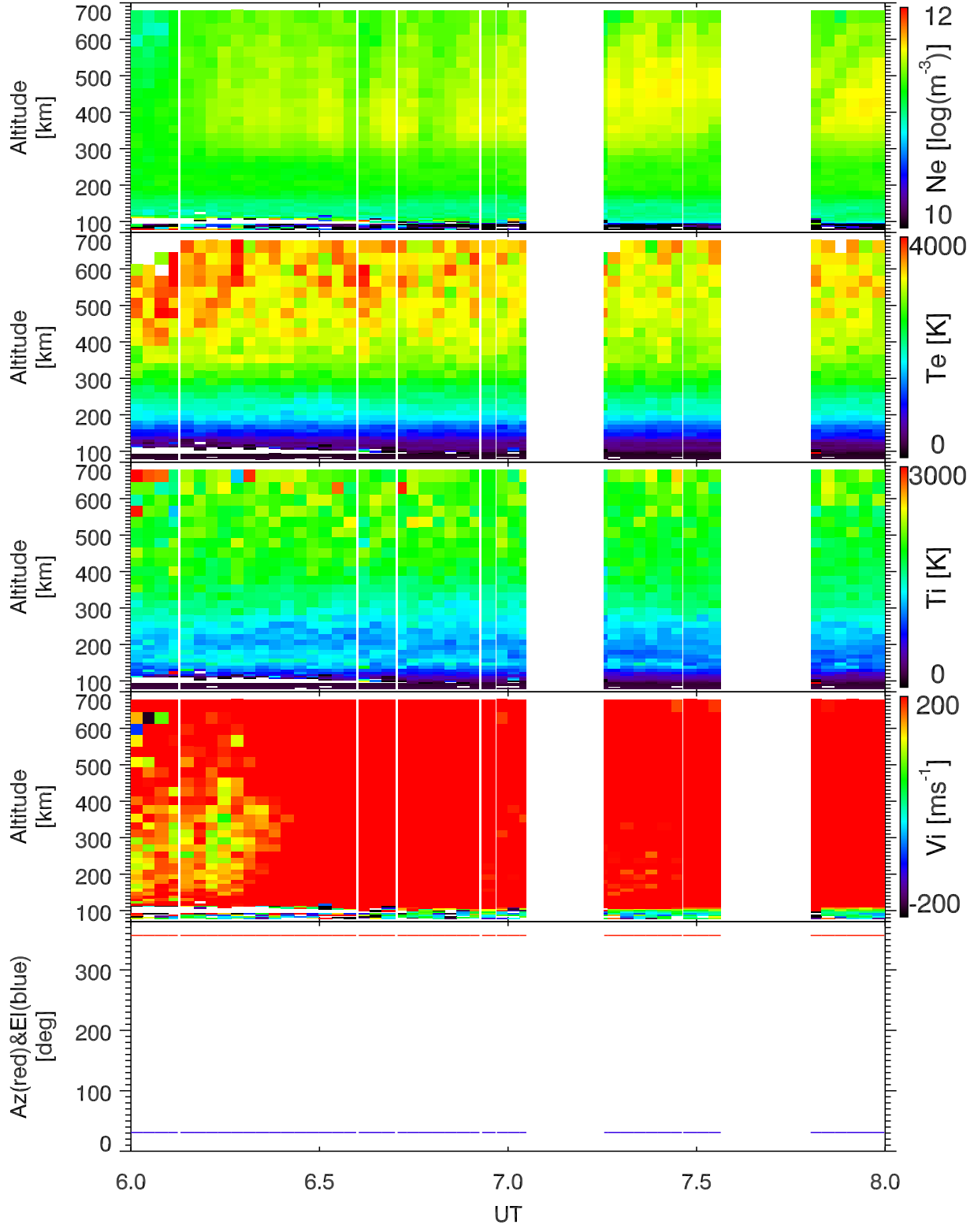
EISCAT 2000-07-20_06_08UT_tau0_120@32m.
