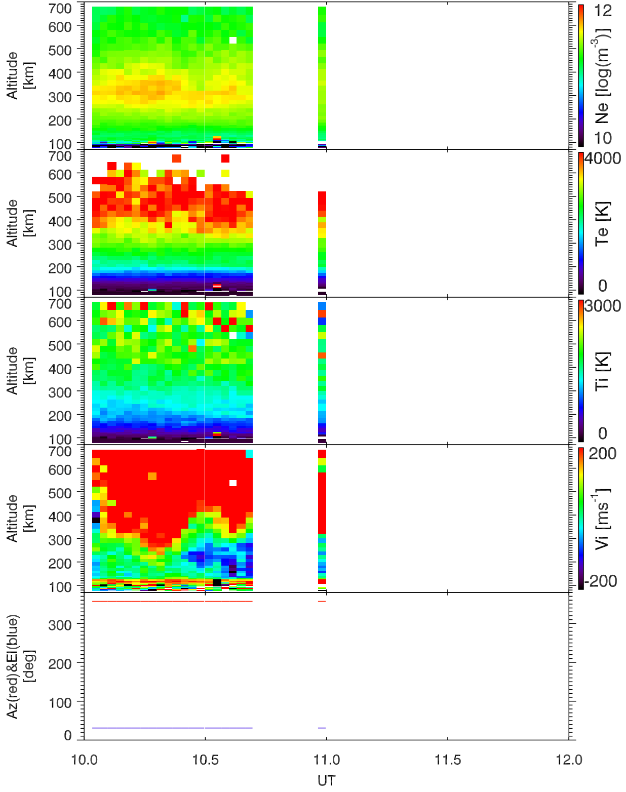
EISCAT 2000-07-23_10_12UT_tau0_120@32m.
