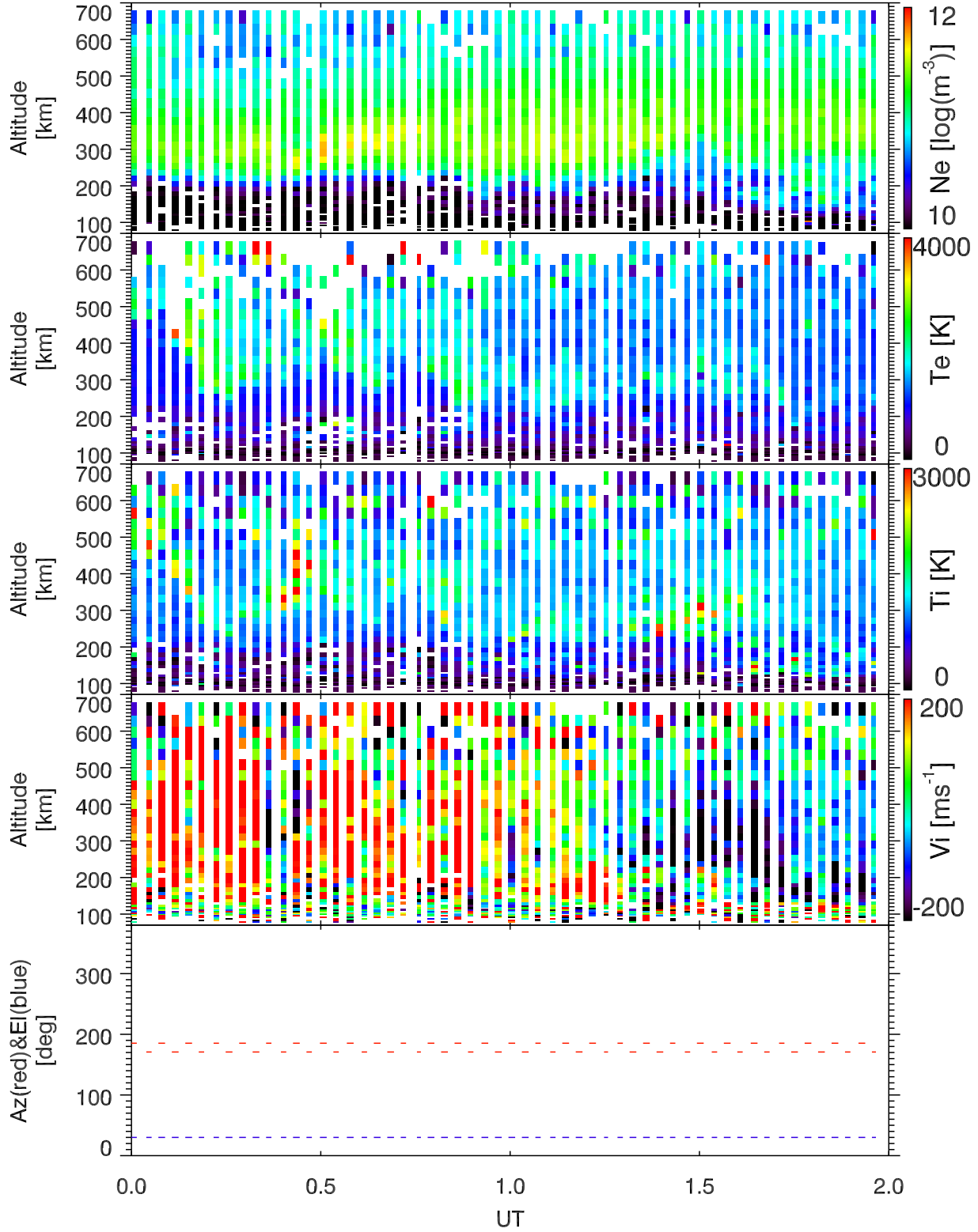
EISCAT 2001-02-19_00_02UT_tau0_ant@32m.
