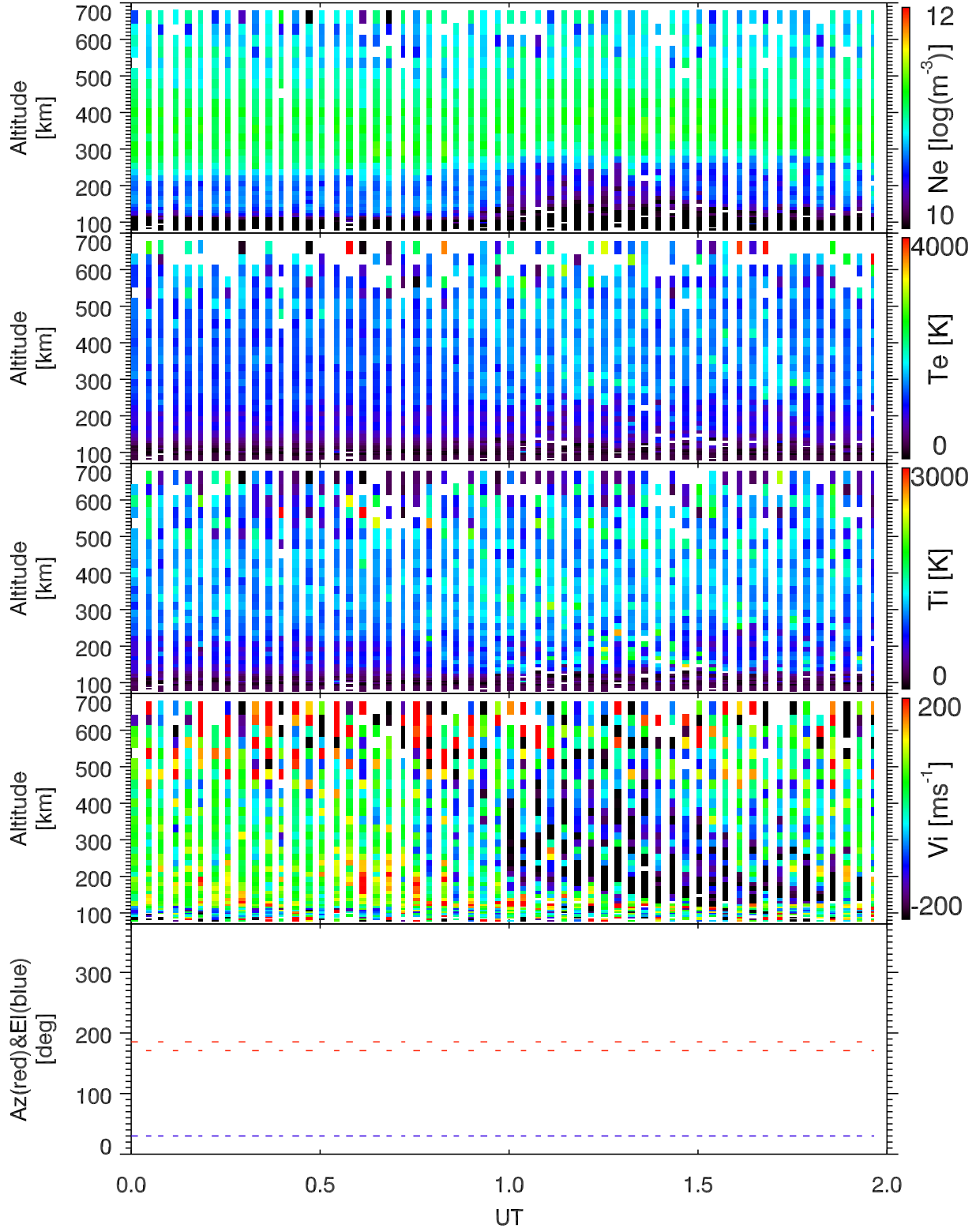
EISCAT 2001-02-22_00_02UT_tau0_ant@32m.
