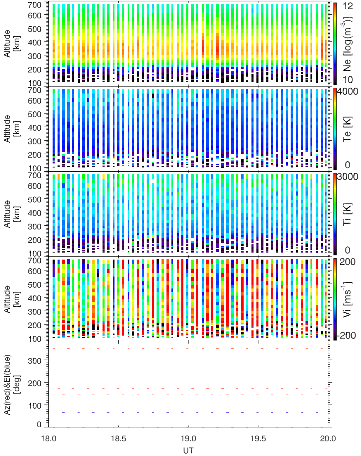
EISCAT 2001-02-22_18_20UT_tau0_ant@32m.
