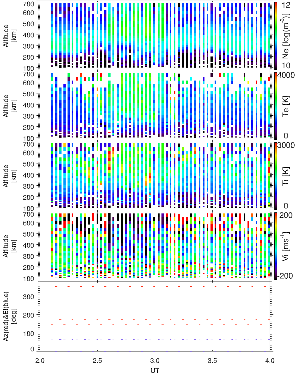
EISCAT 2001-02-23_02_04UT_tau0_ant@32m.
