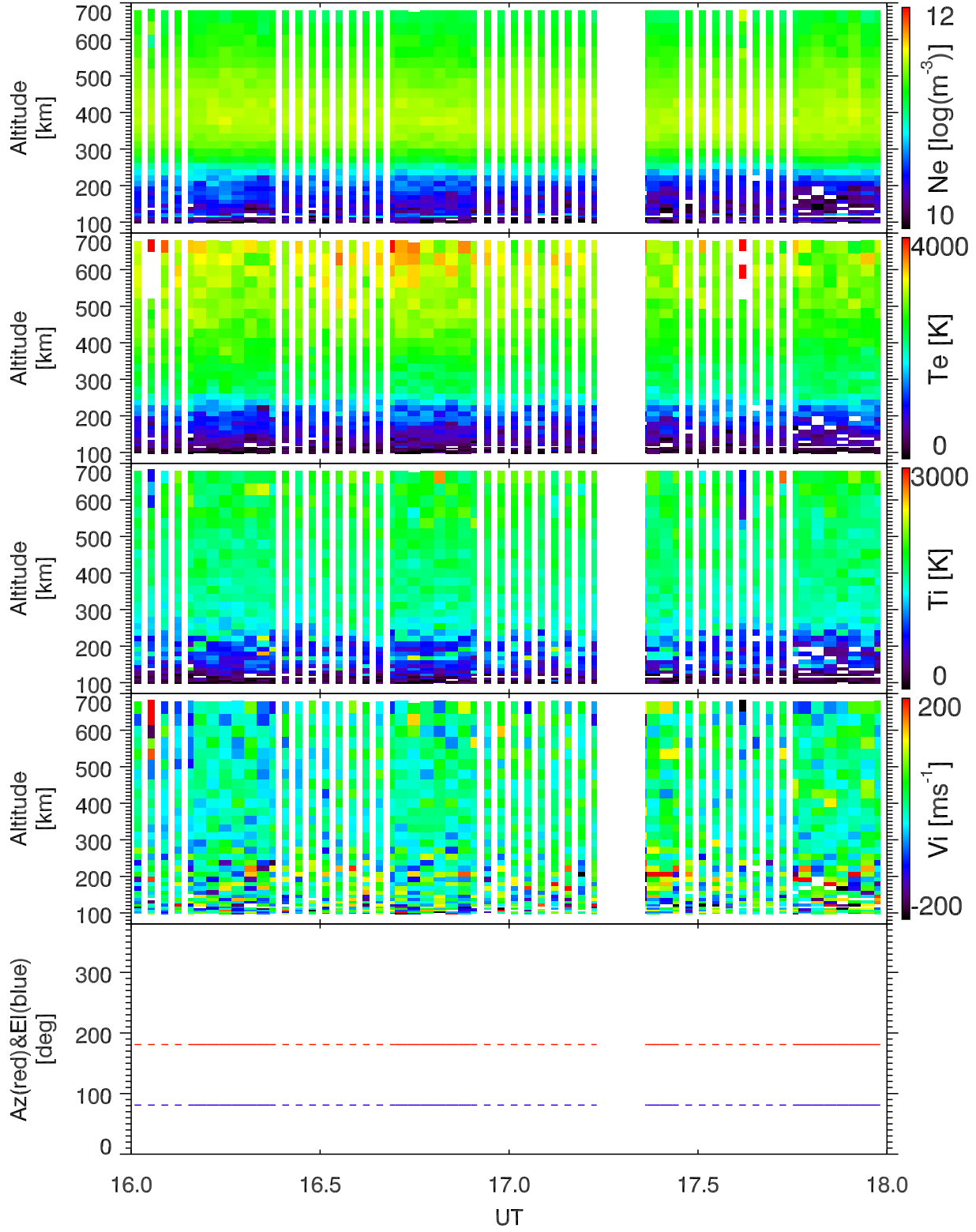
EISCAT 2001-10-01_16_18UT_tau0_120@42m.
