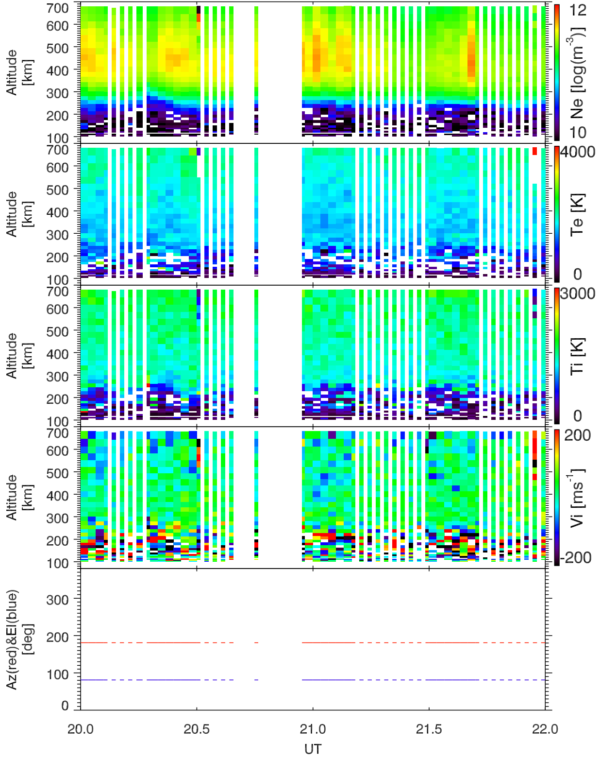
EISCAT 2001-10-01_20_22UT_tau0_120@42m.
