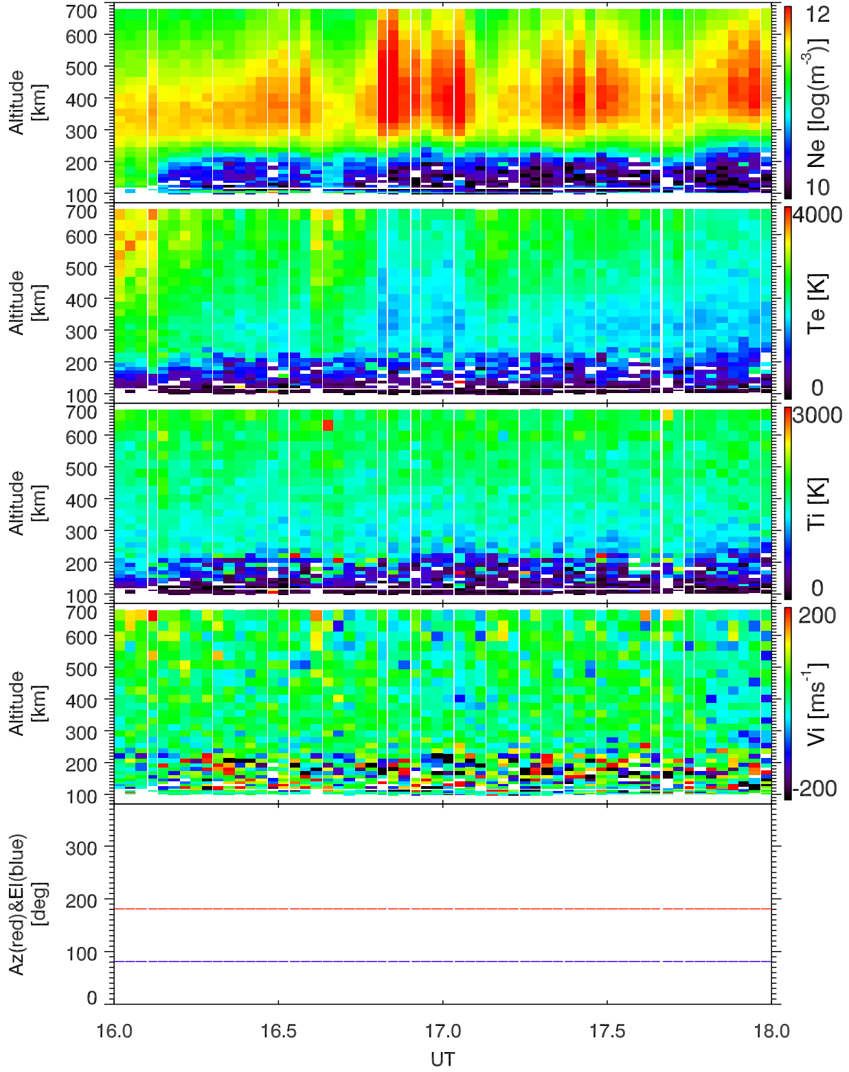
EISCAT 2001-10-08_16_18UT_tau0_all@42m.
