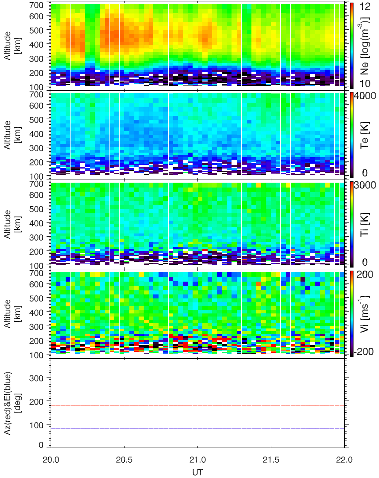
EISCAT 2001-10-08_20_22UT_tau0_all@42m.
