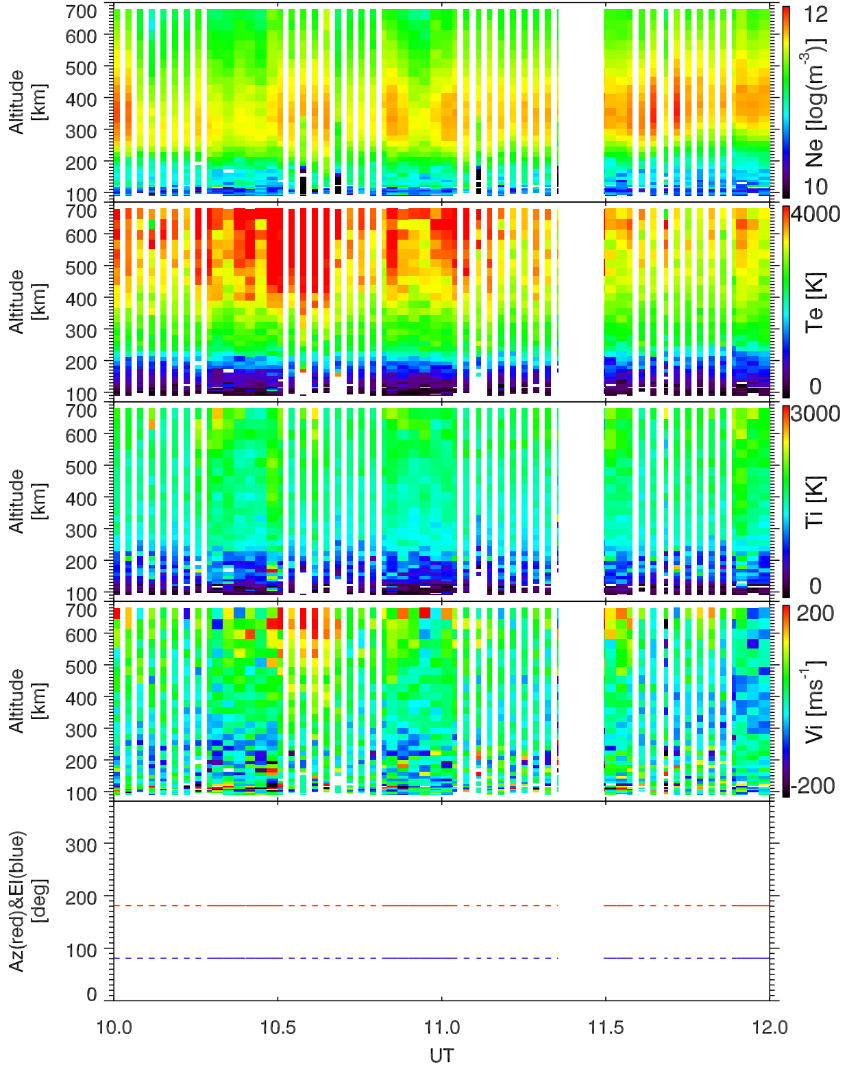
EISCAT 2001-10-09_10_12UT_tau0_120@42m.
